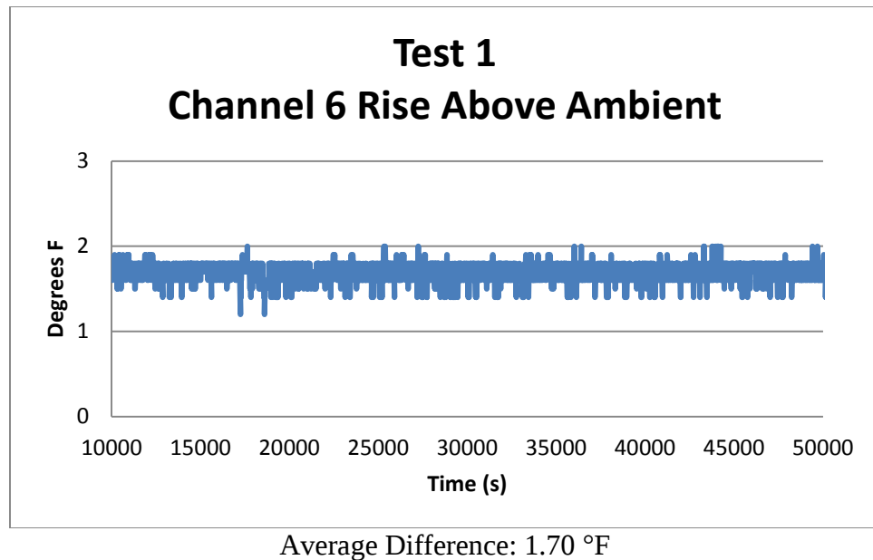
Fig. 9 Difference between screen temperature and ambient through the steady state period of Test 1
