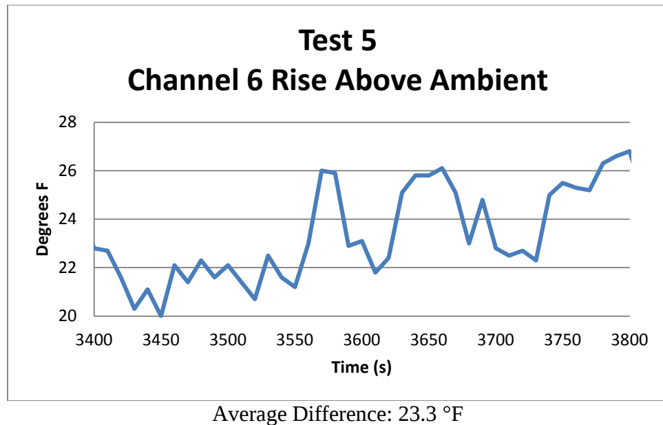
Fig. 21 Difference between screen temperature and ambient through the steady state period of Test 5
