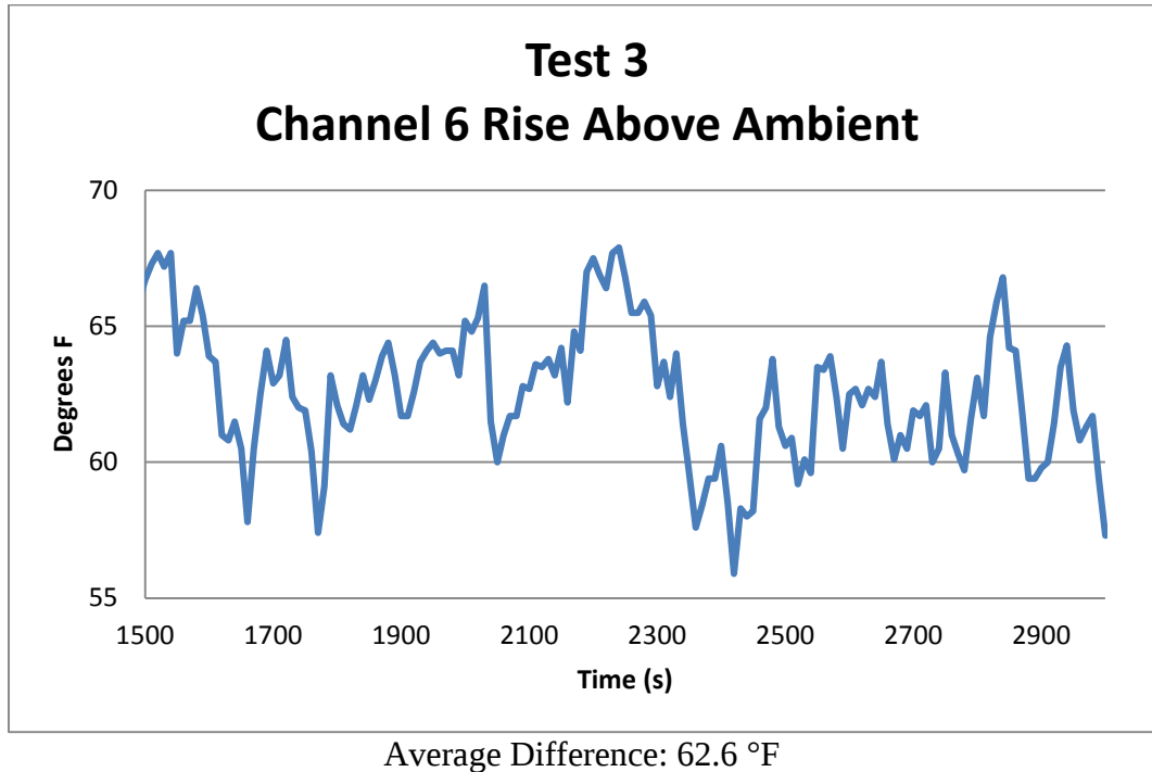
Fig. 15 Difference between screen temperature and ambient through the steady-state period of Test 3
