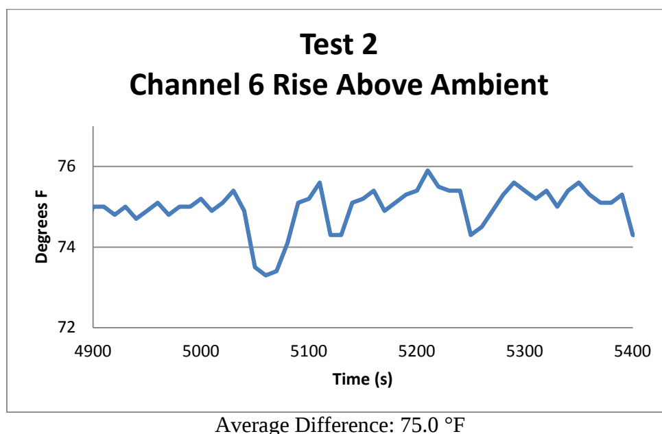
Fig. 12 Difference between screen temperature and ambient through the steady-state period of Test 2
