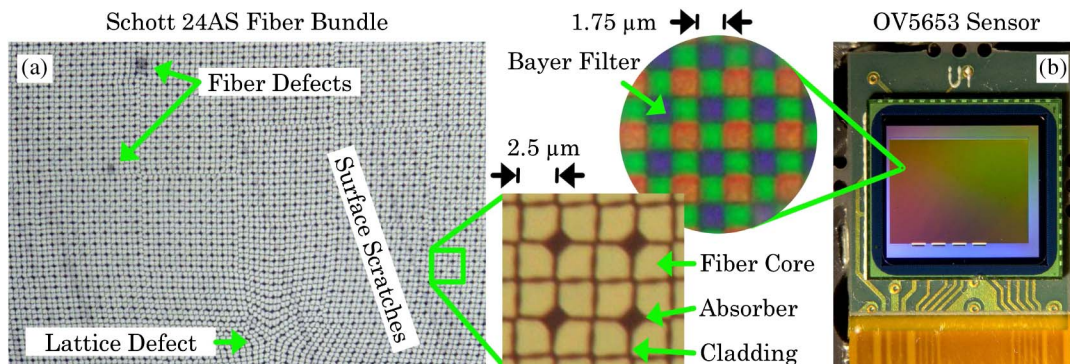
Fig. 3. (a) Fiber bundle structure and defects lead to image artifacts. Fiber absorbers between every other 2.5 \mu\text{m} fiber intersection prevent crosstalk. (b) OV5653 sensor is used to sample the image exiting the fiber bundle. The two magnified inset micrographs are of the same scale.
