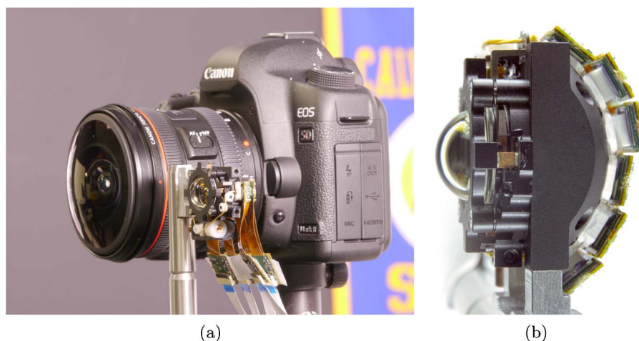
Fig. 4. (a) Side-by-side size comparison of the prototype with an F/4 commercial camera of similar field-of-view. (b) F/1.35 , 30 megapixel, 126^\circ field-of-view fiber-coupled monocentric lens imager prototype.
