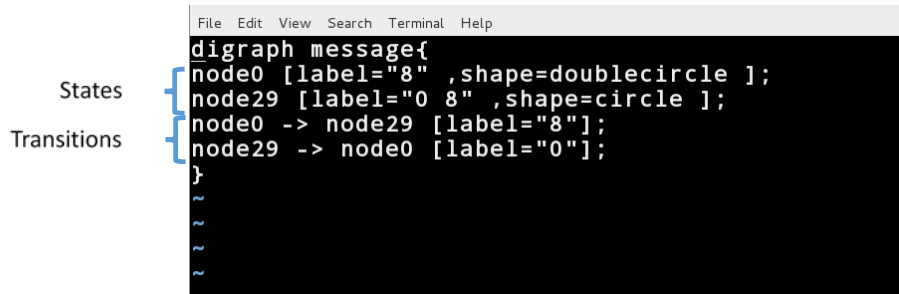
Fig. 16 Ping “labeledStateMachine.dot” file
