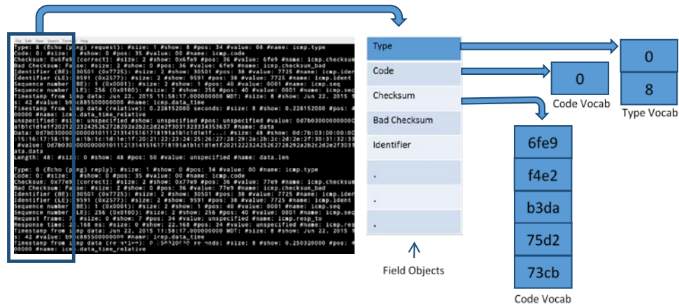
Fig. 14 Vocabulary generation
