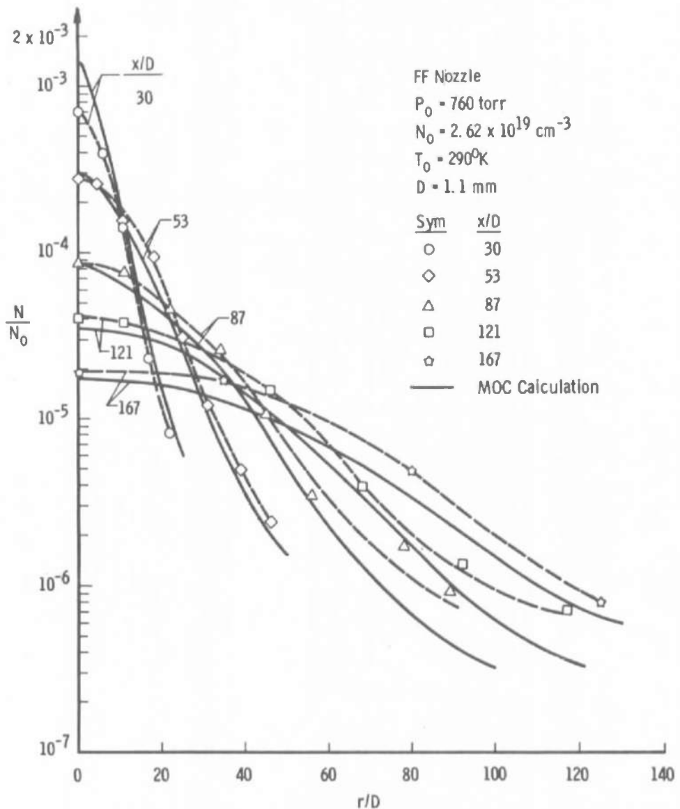
Figure 26. Electron beam radial density profiles, P_0 = 760 torr.
