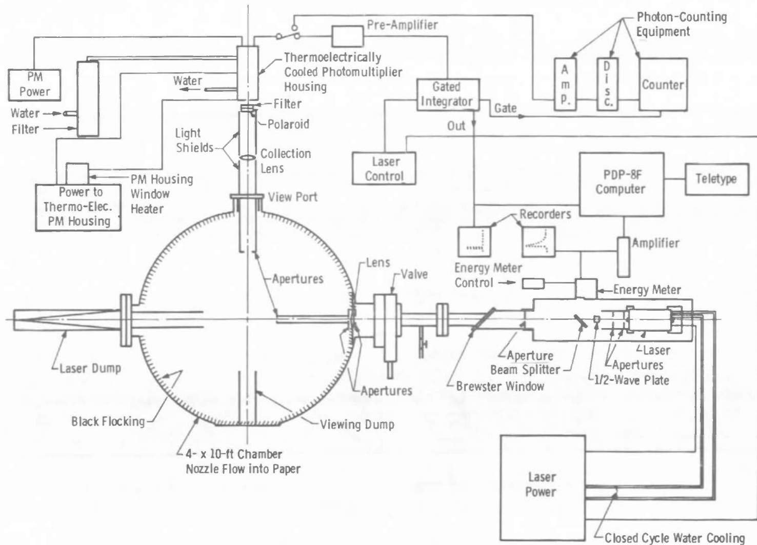
Figure 7. Optical and electronic arrangement for Rayleigh scattering measurements.
