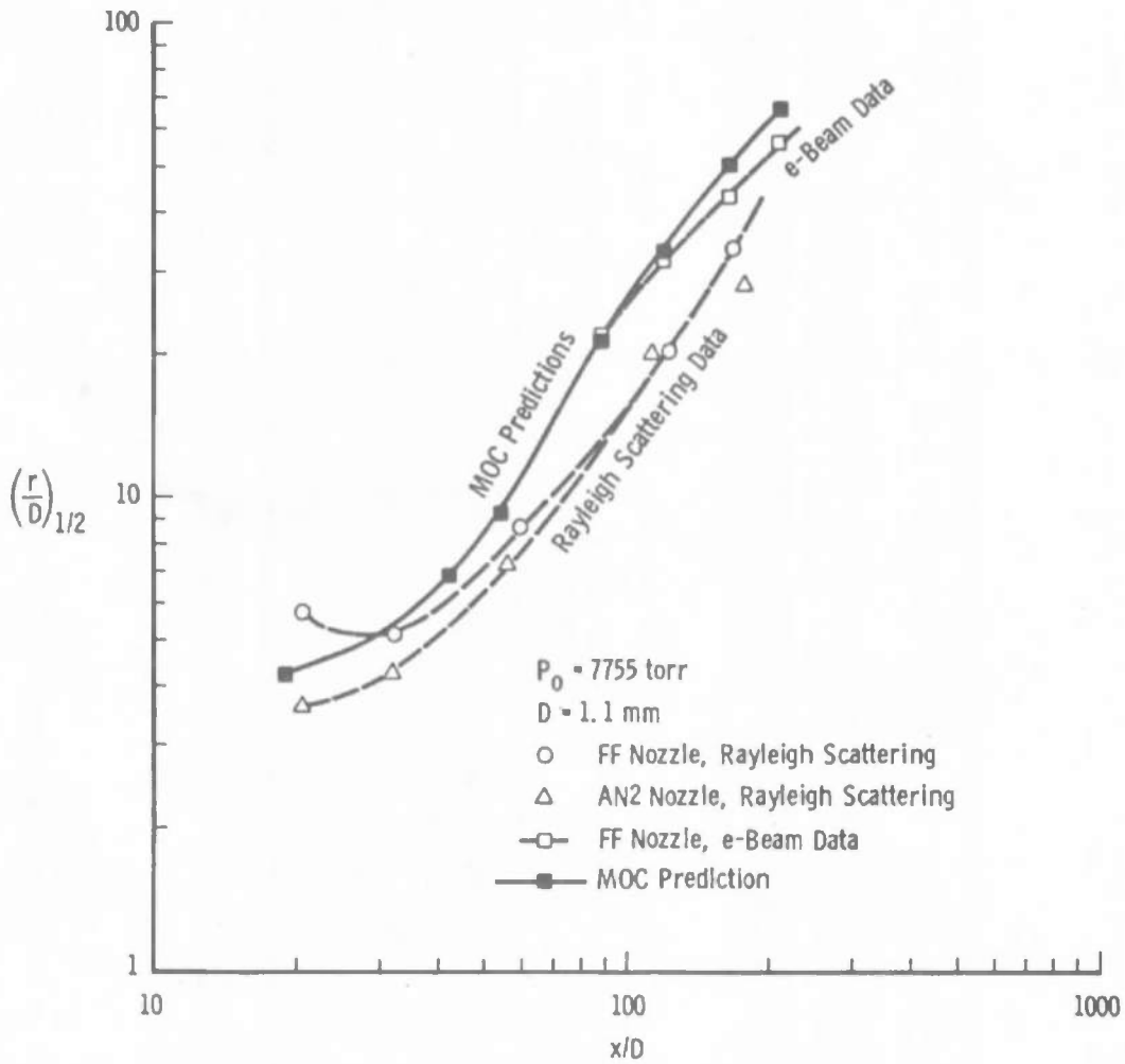
Figure 51. Variation of half-width, half-maximum points of \langle Na^6 \rangle and N with axial distance.
