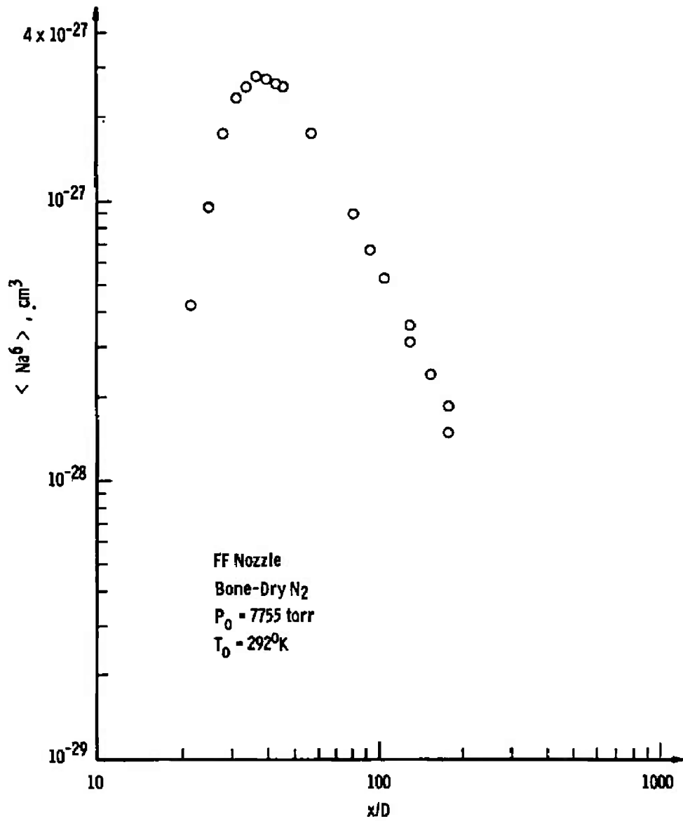
Figure 39. Experimental Rayleigh scattering axial profile, FF nozzle, P 0 = 7755 torr.
