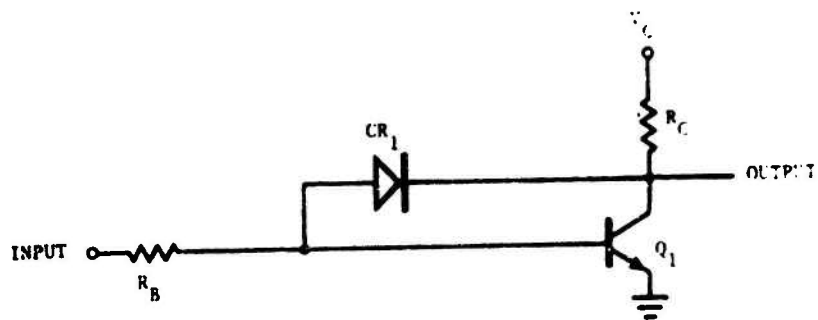
(a) Collector-Base Clamp
