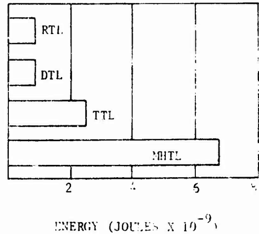
Figure 4-6. Comparison of Logic Family Upset Threshold
