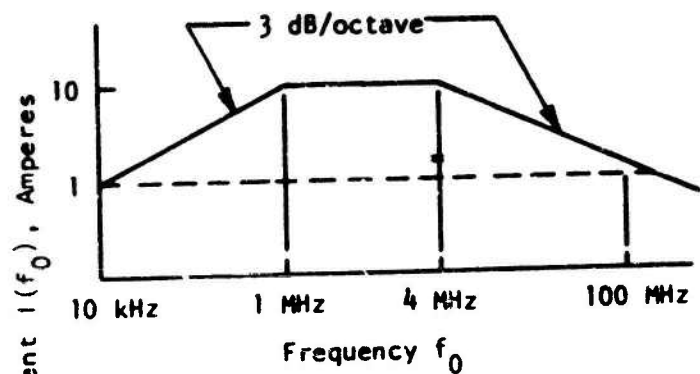
Peak Core Current Requirement for General Electronic Equipment
