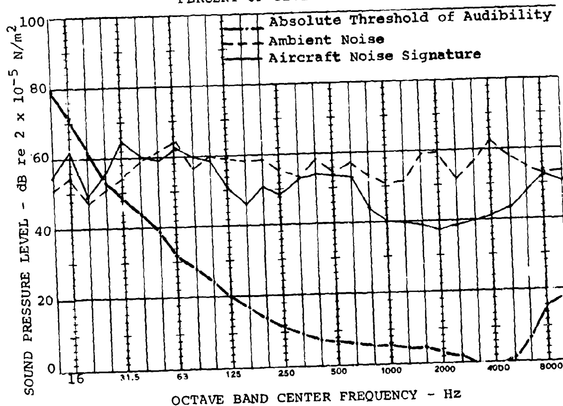
Figure 29. Observation and Acoustical Data - Run 12.
