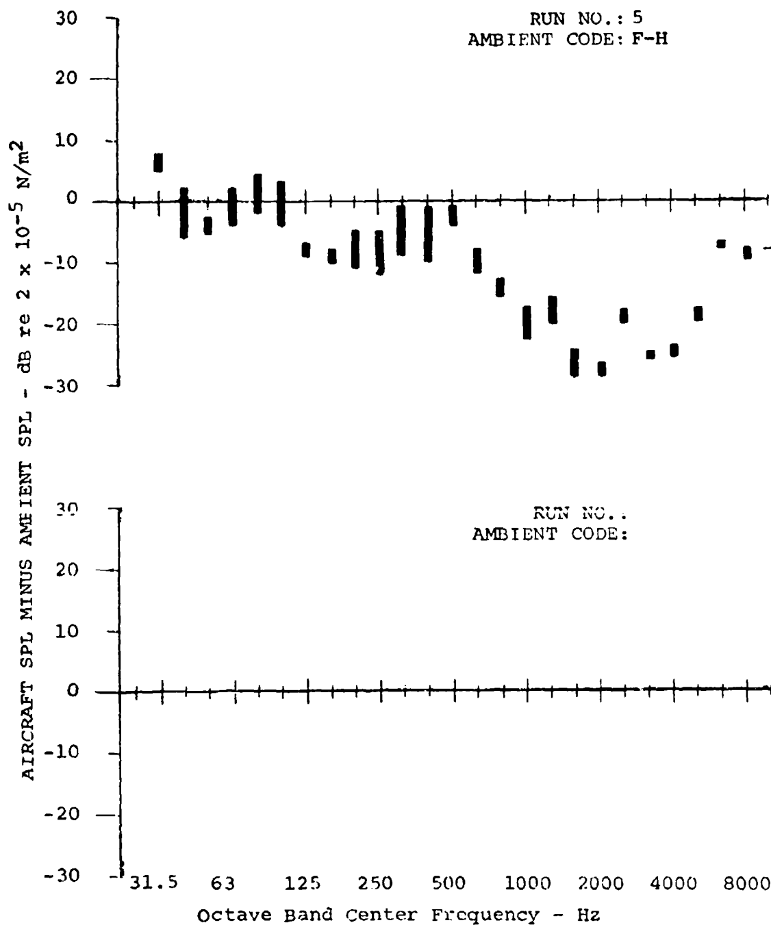
Figure 60. Detection Results With Flat, High-Level Ambient.
