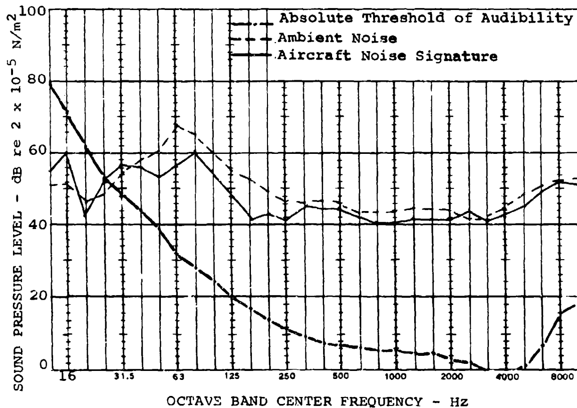
Figure 41. Observation and Acoustical Data - Run 24.
