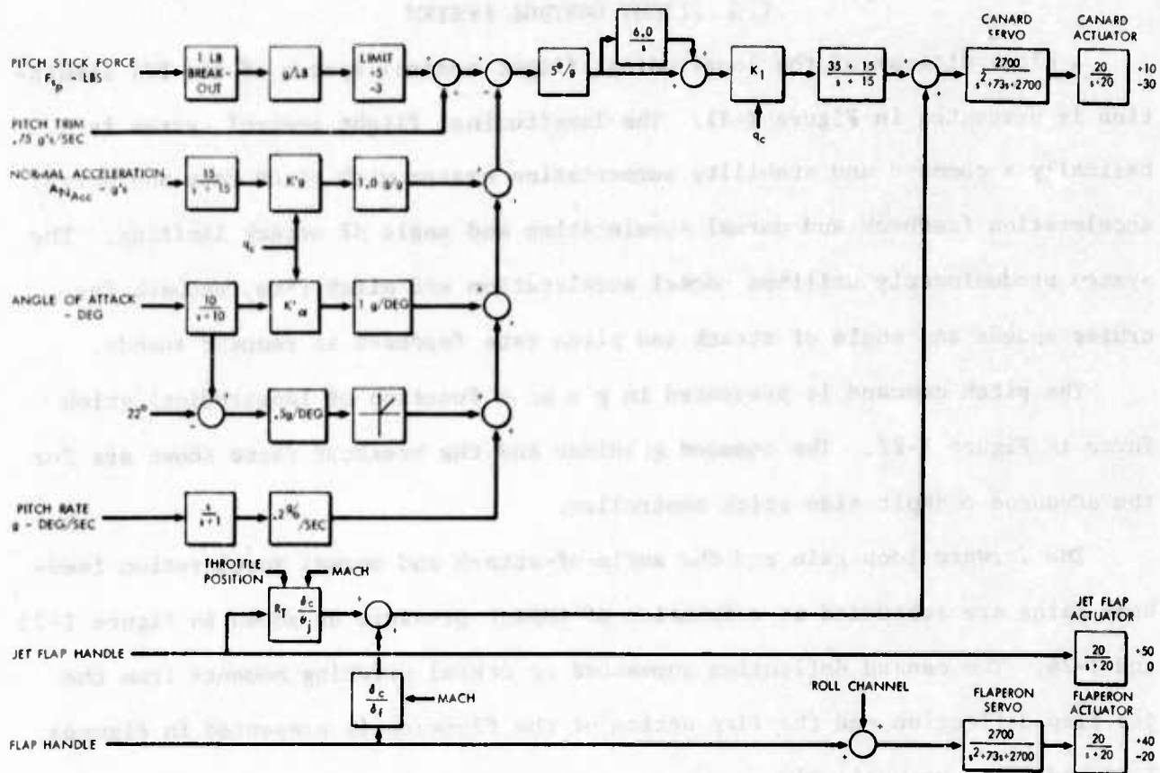
Figure I-21 Longitudinal Flight Control System
