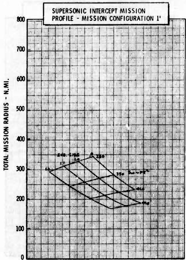
Figure H-55c LWA Mission/Configuration Tradeoff Parametric Data
