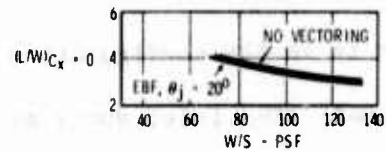
Figure B-35 EBF In-Flight Performance Potential
