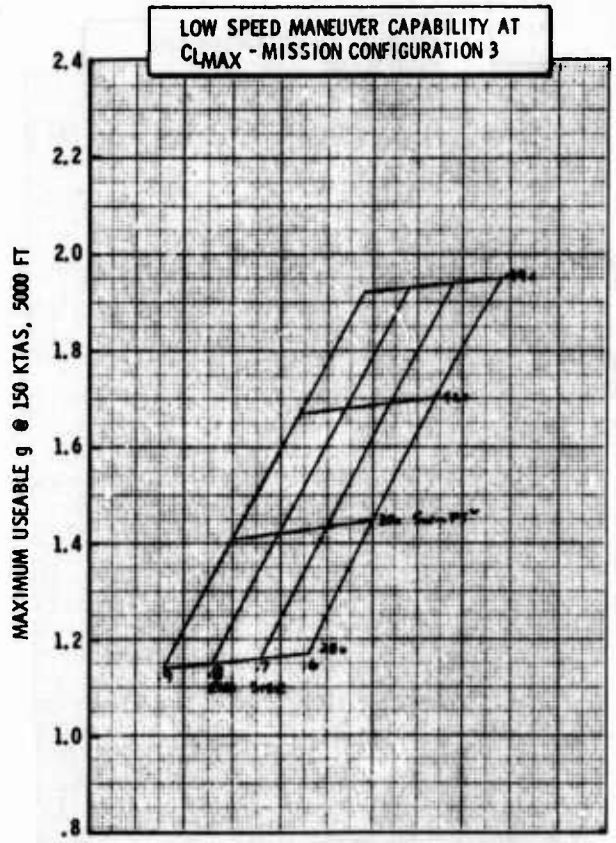
Figure H-30a LWA Mission/Configuration Tradeoff Parametric Data
