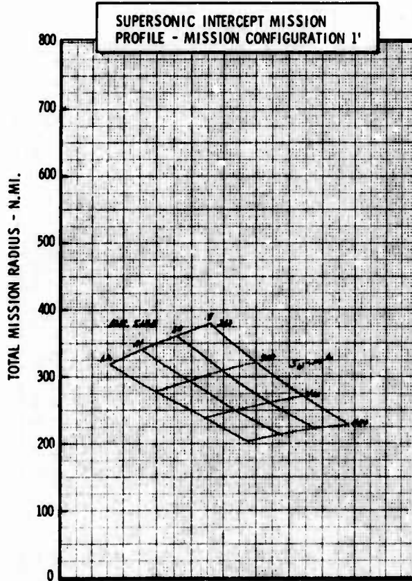
Figure H-50c LWA Mission/Configuration Tradeoff Parametric Data
