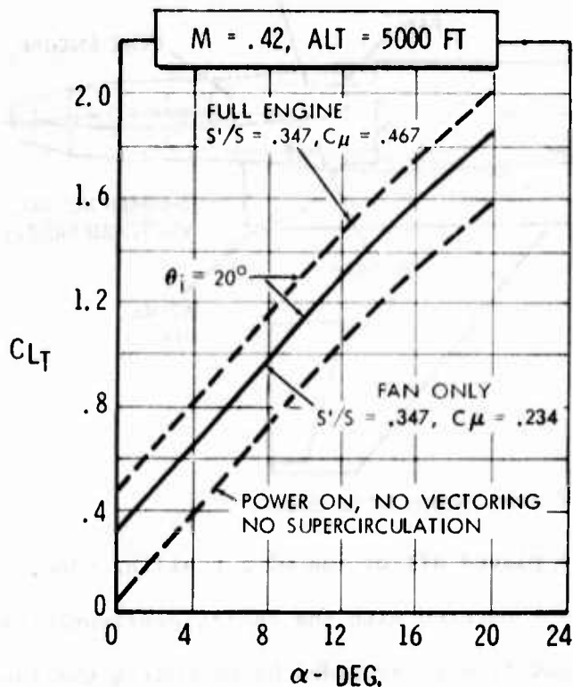
Figure B-32 Fan-Air-Only VT/SC Aerodynamic Performance Potential
