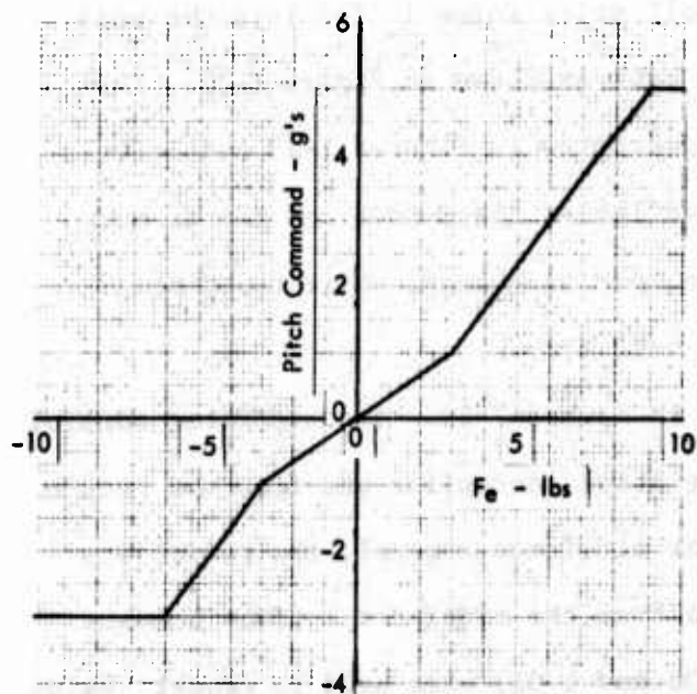
Figure I-22 Pitch Acceleration Command
