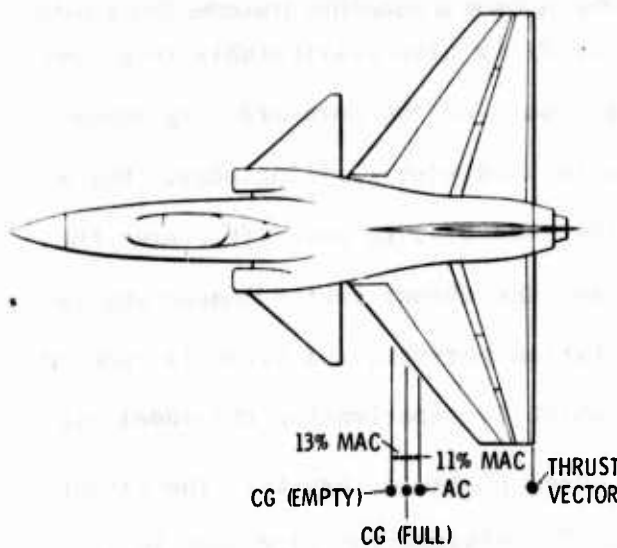
Figure D-32 Initial VT/SC Configuration Severely Limited Trimmable Thrust Vector Angle
