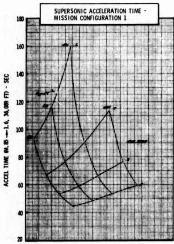
Figure H-29b LWA Mission/Configuration Tradeoff Parametric Data
