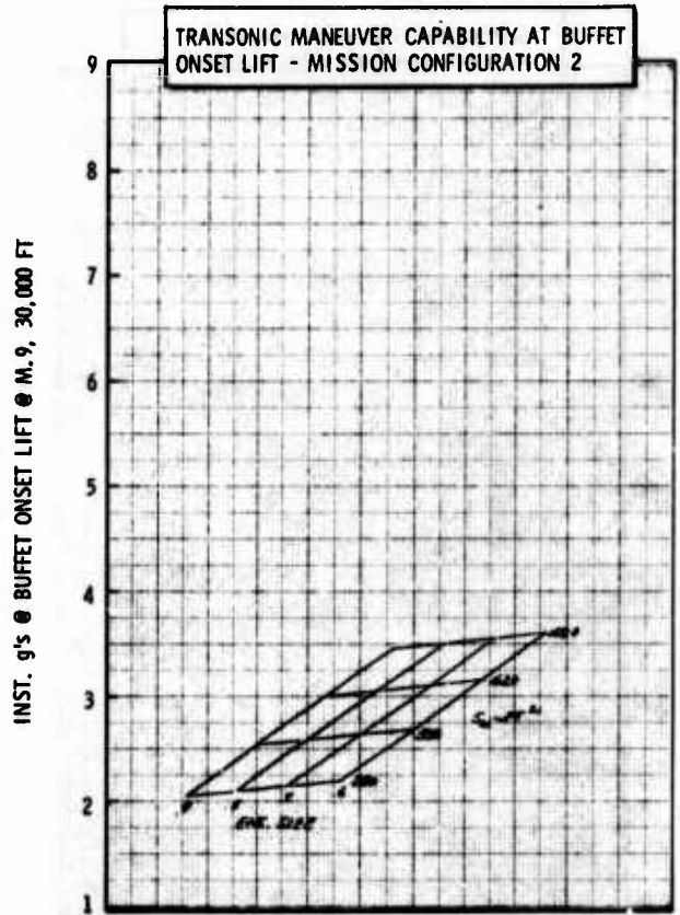
Figure H-7b LWA Mission/Configuration Tradeoff Parametric Data
