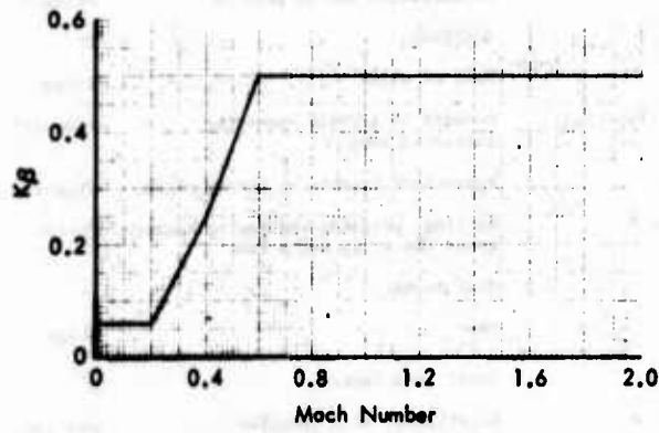
Figure I-29 Rudder Forward Loop Gain and Sideforce Mode Feedback Gain
