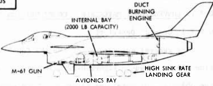
Figure D-22 LWA Conventional Reference Configuration 26B
