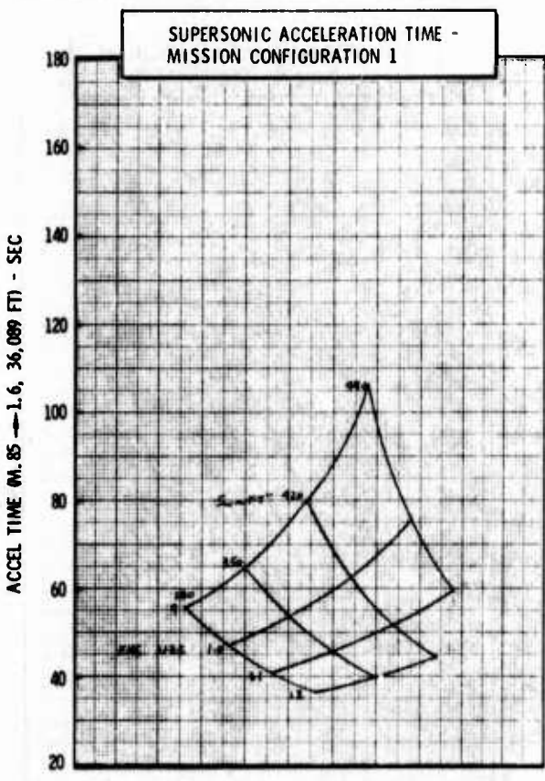
Figure H-28b LWA Mission/Configuration Tradeoff Parametric Data
