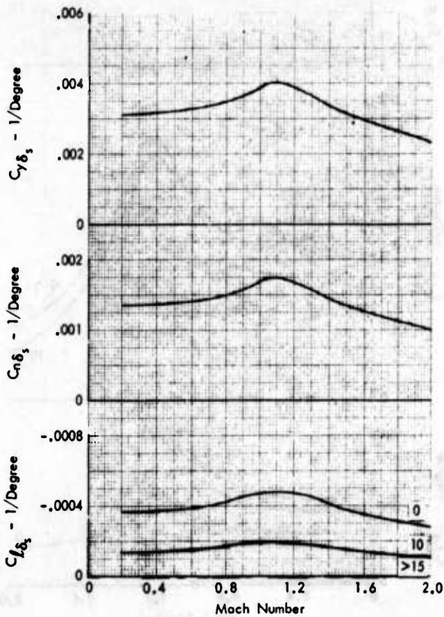
Figure 1-15 Sideforce Derivatives
