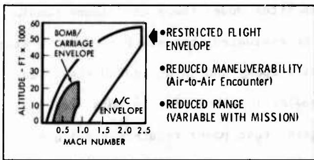
Figure A-33 External Pylon Mounted Weapons can Limit Aircraft Performance
