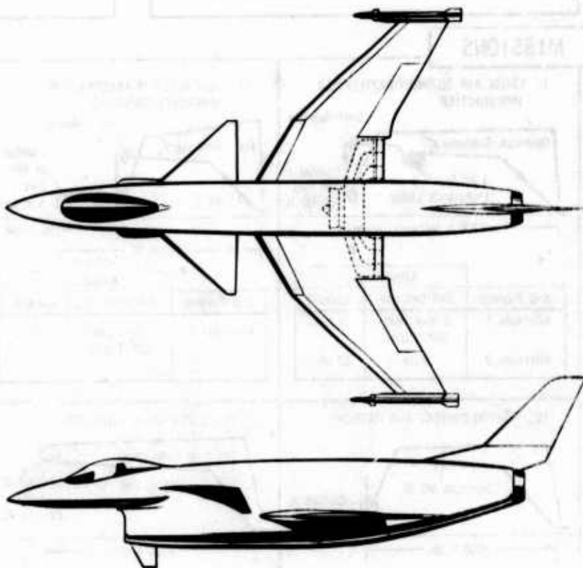
Figure 1-2 LWA Configuration 29
