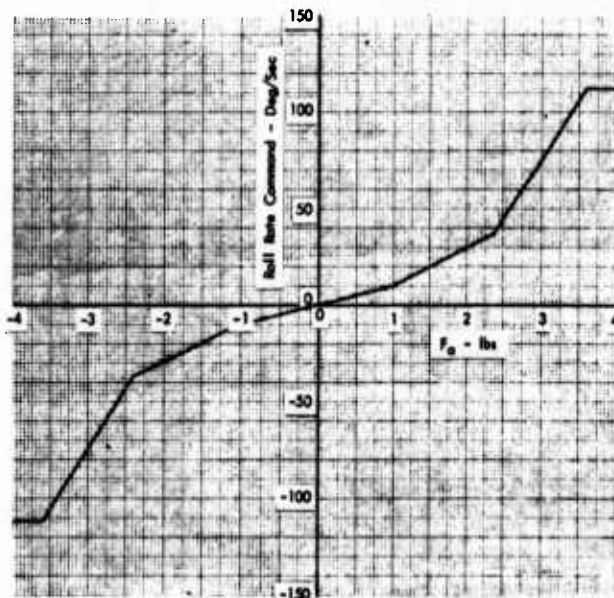
Figure I-28 Roll Rate Command
