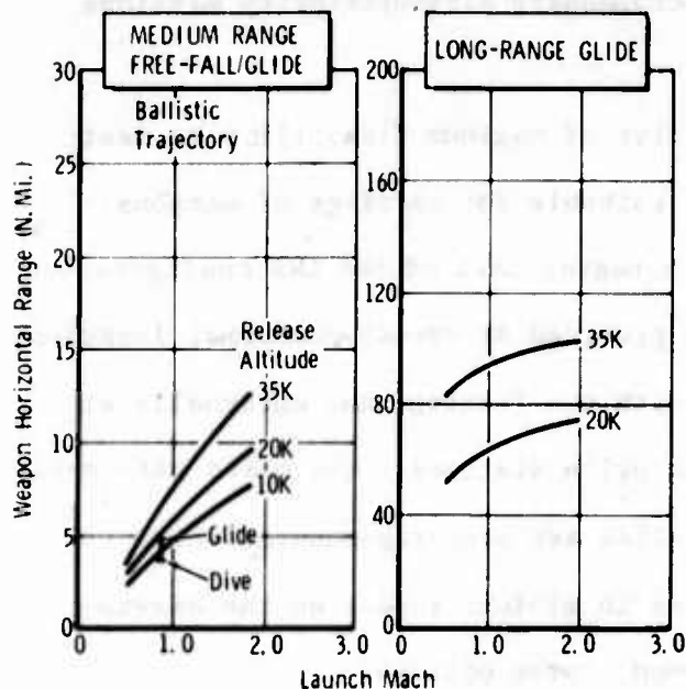
Figure D-3 LWA can be an Effective Booster for Unpowered Stand-off Weapons
