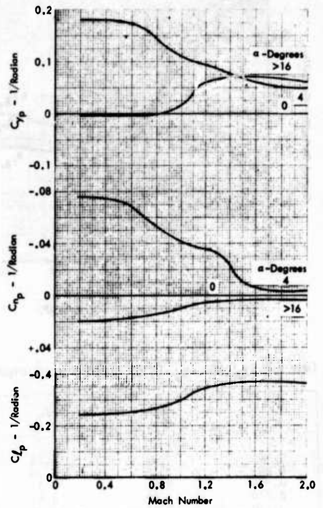
Figure 1-18 Roll Rate Derivatives
