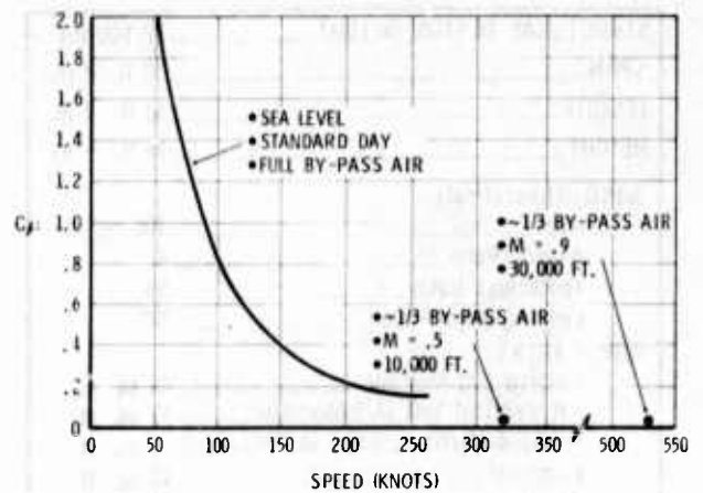
Figure D-41 Configuration 28 C_{\mu} at Selected Conditions
