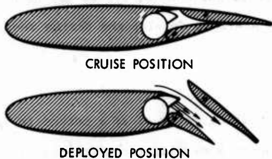
Thick S/C Airfoil could be Advantageous
