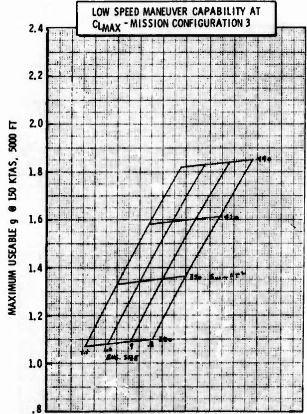
Figure H-18a LWA Mission/Configuration Tradeoff Parametric Data
