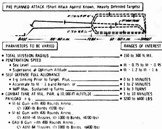
Figure D-52 LWA Employment for Interdiction/Strike Role is Basis for Pre-Planned Attack Mission
