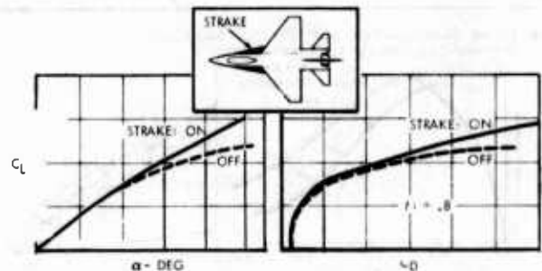
Figure A-9 Wing-Body Design Integration can Improve L/D at High Angles of Attack
