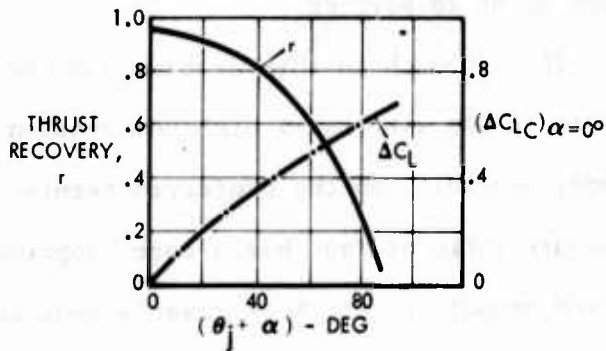
Figure B-12 Jet Flap Performance is Function of Jet Angle, \theta_j
