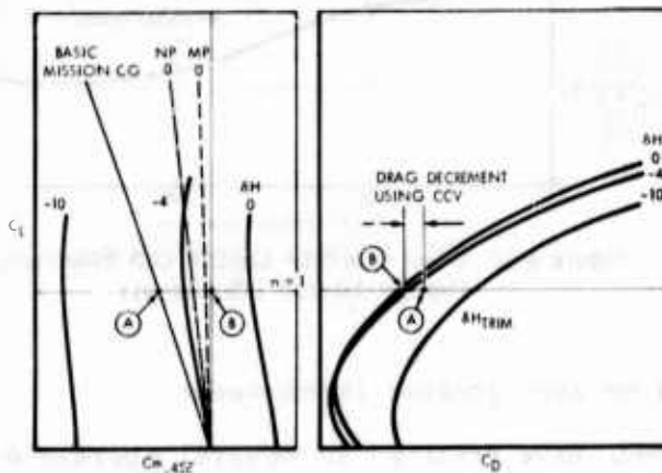
Figure A-10 Cruise Drag Reduction Through CCV
