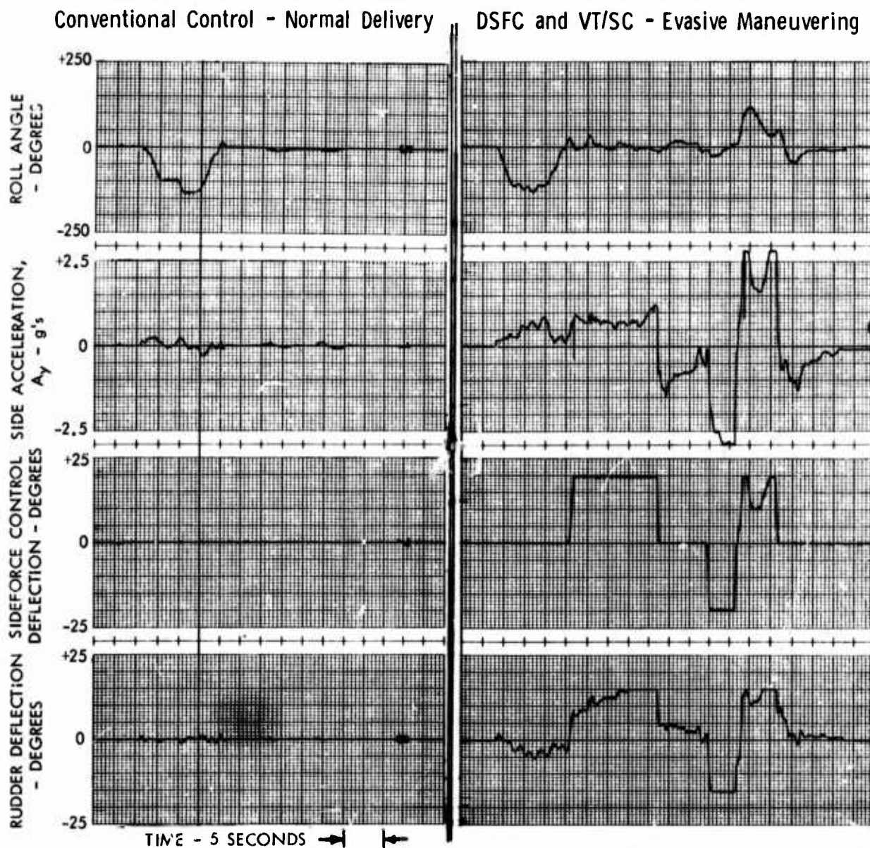
Figure 4-1 Weapon Delivery Profile Comparison Shows Typical Evasive Maneuver Using VT/SC and DSFC
