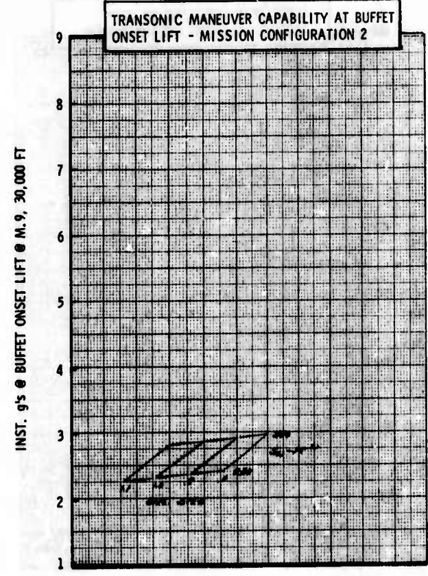
Figure H-19b LWA Mission/Configuration Tradeoff Parametric Data
