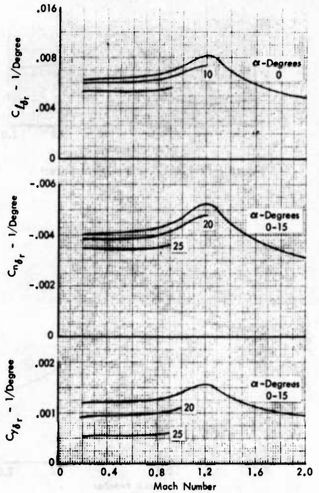
Figure 1-16 Vertical Tail Derivatives
