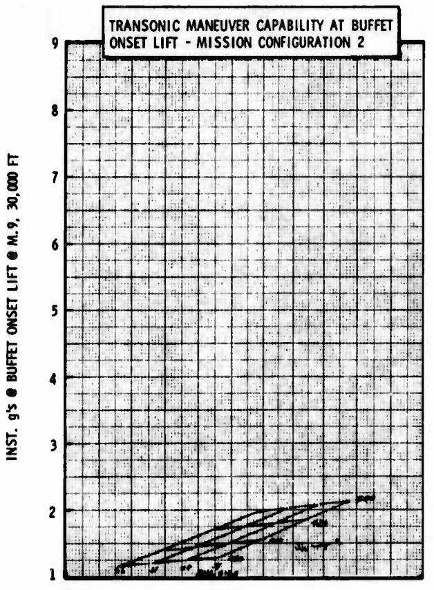
Figure H-49b LWA Mission/Configuration Tradeoff Parametric Data
