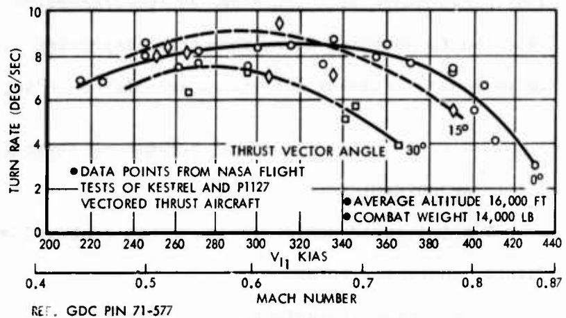
Figure A-1 Vectored Thrust Can Decrease Landing Distance and Increase Turn Rate
