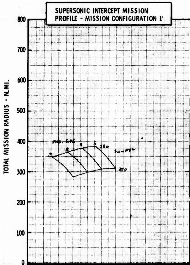
Figure H-37c LWA Mission/Configuration Tradeoff Parametric Data
