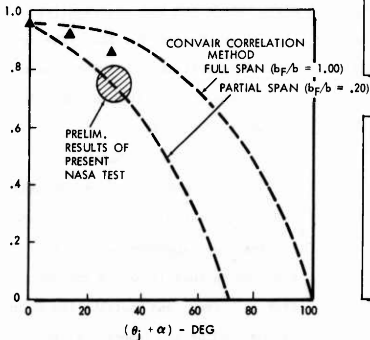
Figure F-1 VT/SC Thrust Recovery Picture is Cloudy
