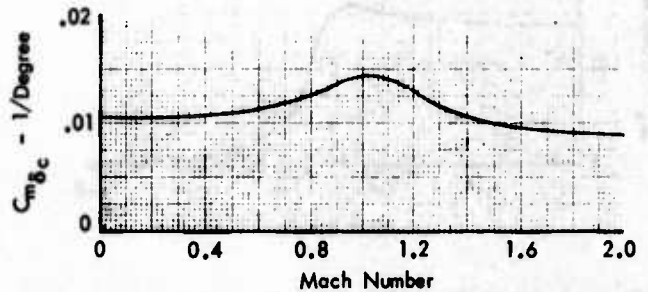
Figure 1-9 Canard Lift and Moment Curves
