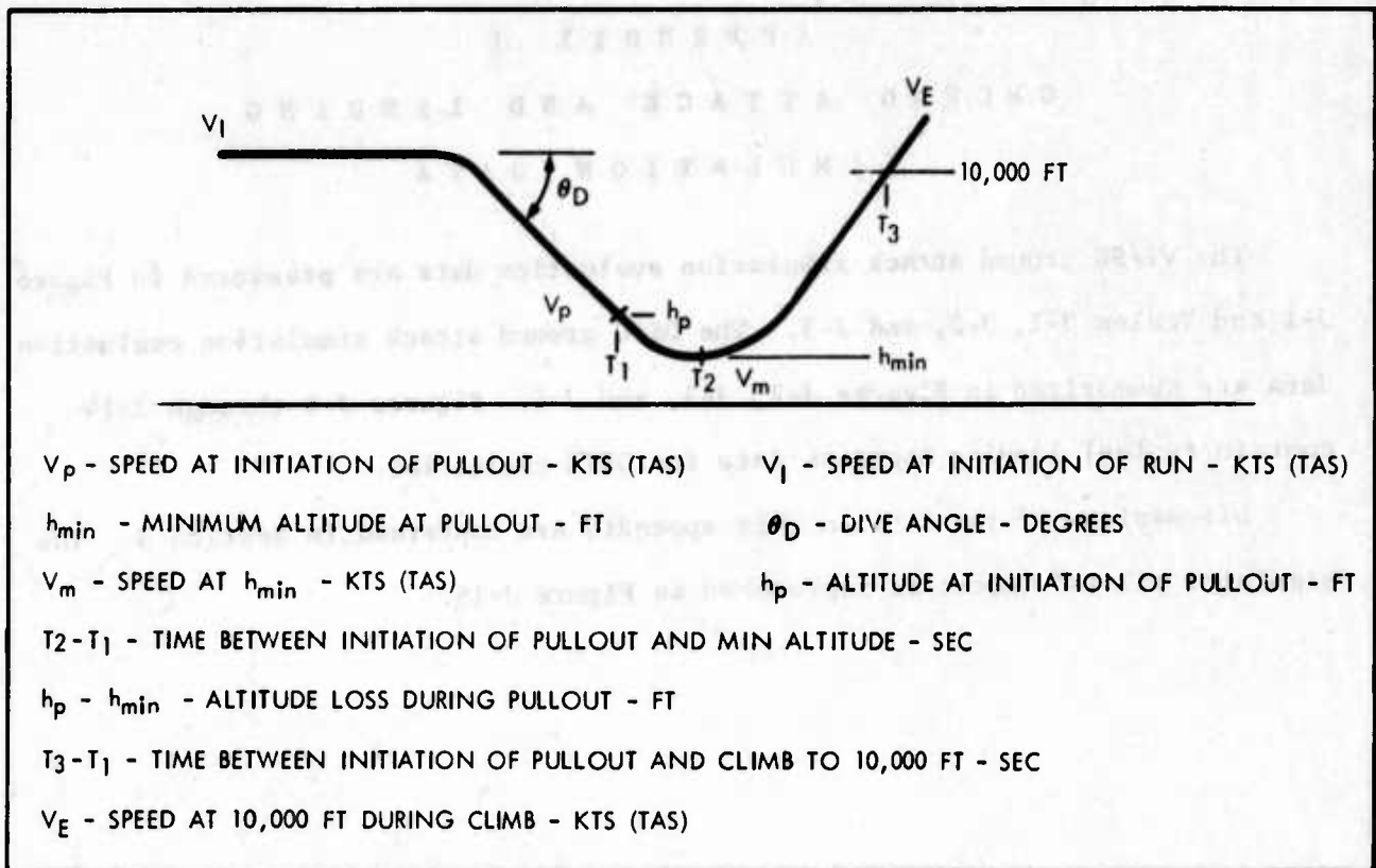
Figure J-1 VT/SC Ground Attack Simulation Geometry
