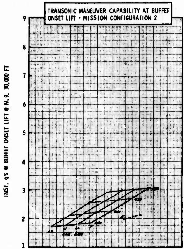
Figure H-51) LWA Mission/Configuration Tradeoff Parametric Data
