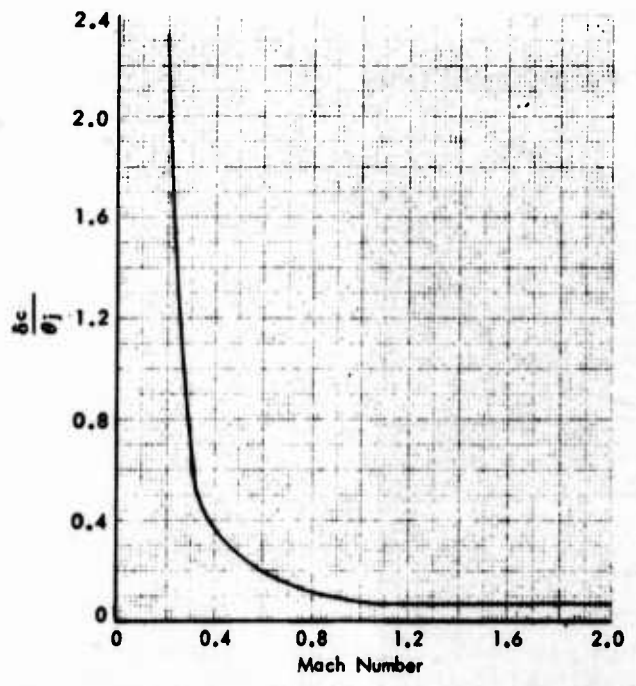
Figure 1-25 Jet Flap/Canard Interconnect Gain
