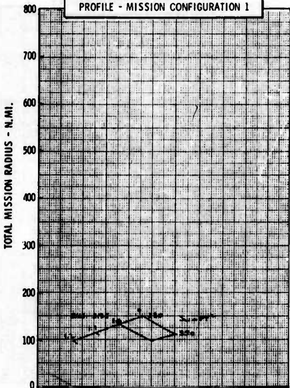
Figure H-28c LWA Mission/Configuration Tradeoff Parametric Data
