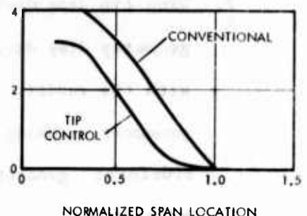
Figure A-11 Maneuver Load Control Can Reduce Weight
