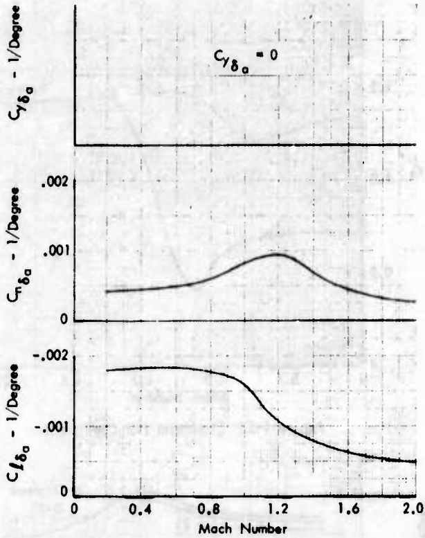
Figure 1-14 Aileron Derivatives
