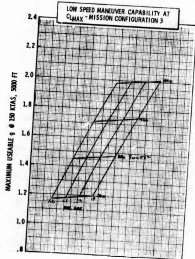
Figure H-22a LWA Mission/Configuration Tradeoff Parametric Data
