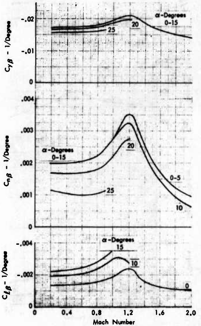
Figure I-13 Sideslip Derivatives
