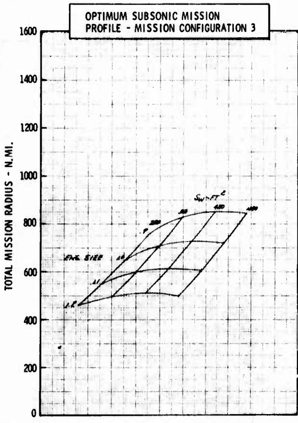
Figure H-47a LWA Mission/Configuration Tradeoff Parametric Data
