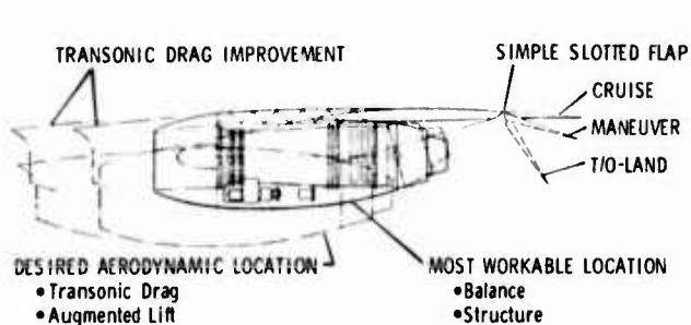
Figure B-37 Desired Engine/Wing Location for EBF Compromised by Required Aft Shift of CG
