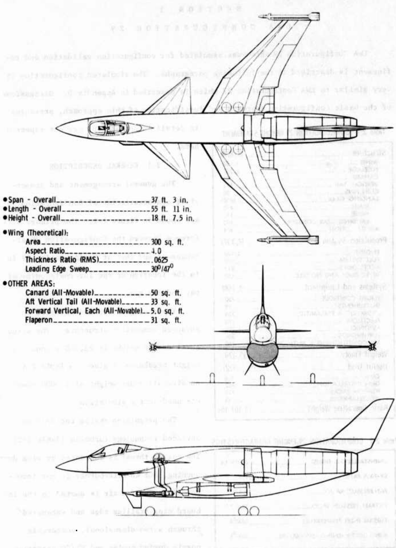
Figure 2-1 Configuration 29 General Arrangement
