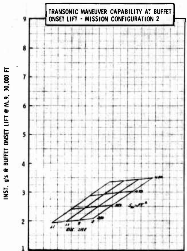
Figure H-42b LWA Mission/Configuration Tradeoff Parametric Data
