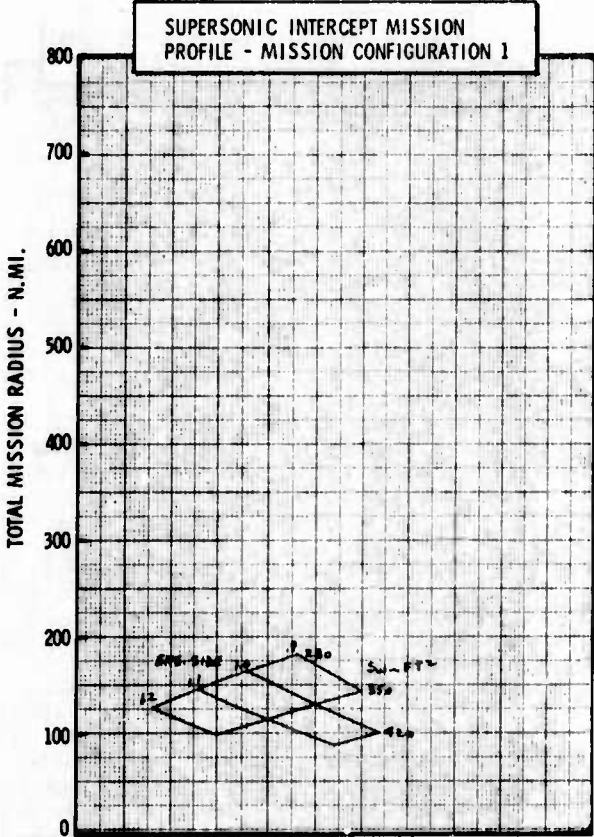
Figure H-27c LWA Mission/Configuration Tradeoff Parametric Data
