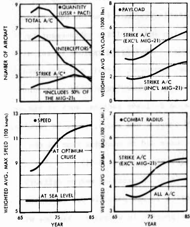
Figure A-47 Soviet Aircraft Trends
