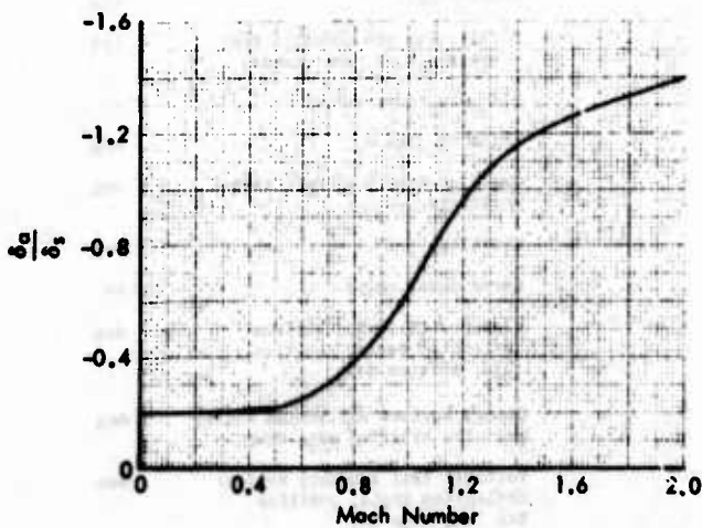
Figure I-31 Rudder/Flaperon and Sideforce/Flaperon Interconnect Gains
