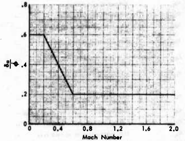
Figure I-30 Sideforce/Rudder Interconnect Gain and Flaperon (Aileron) Forward Loop Gain
