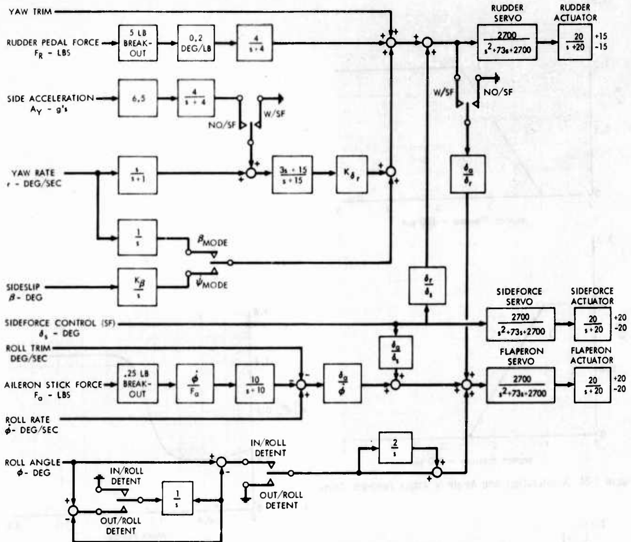
Figure I-27 Lateral-Directional Flight Control System
