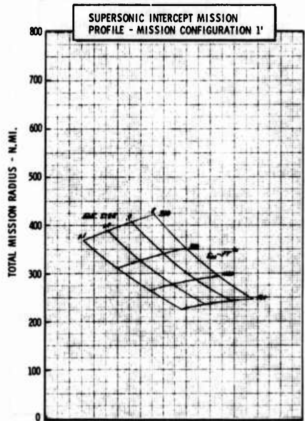
Figure H-42c LWA Mission/Configuration Tradeoff Parametric Data
