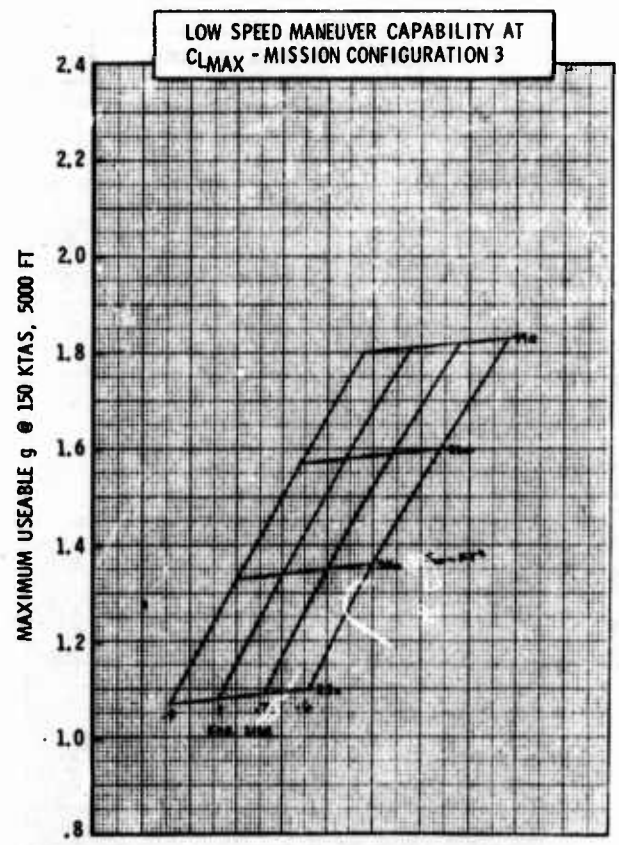
Figure H-4a LWA Mission/Configuration Tradeoff Parametric Data
