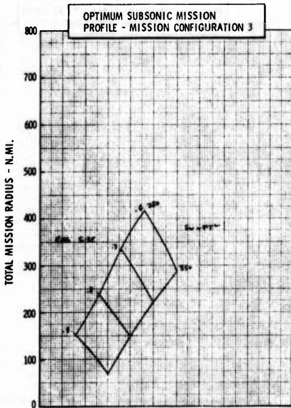
Figure H-10a LWA Mission/Configuration Tradeoff Parametric Data
