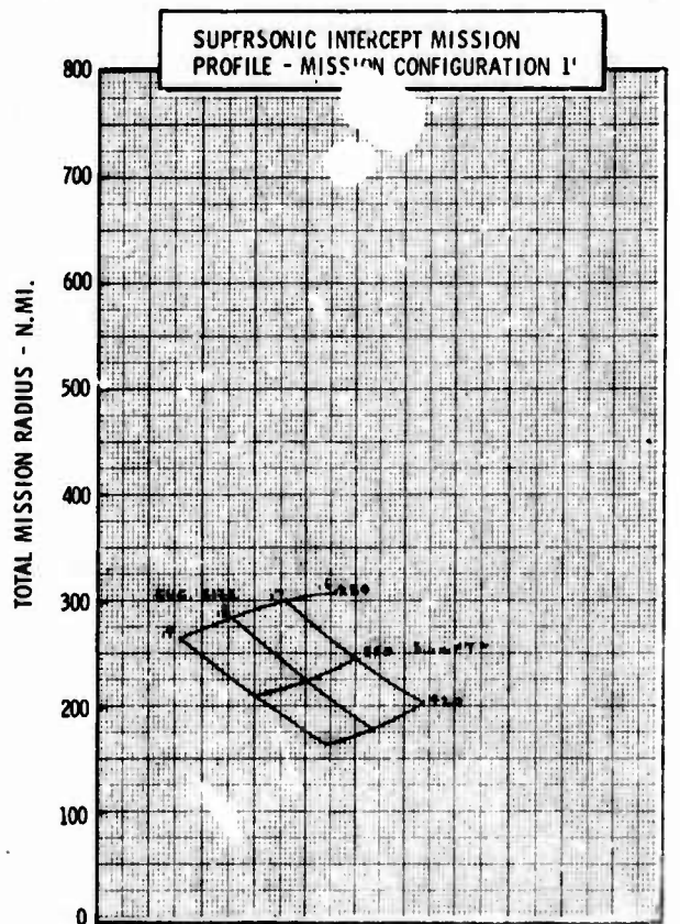
Figure H-4c LWA Mission/Configuration Tradeoff Parametric Data
