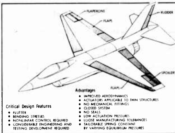
Figure A-26 Flexible Structures Applied to Aerodynamic Surfaces
