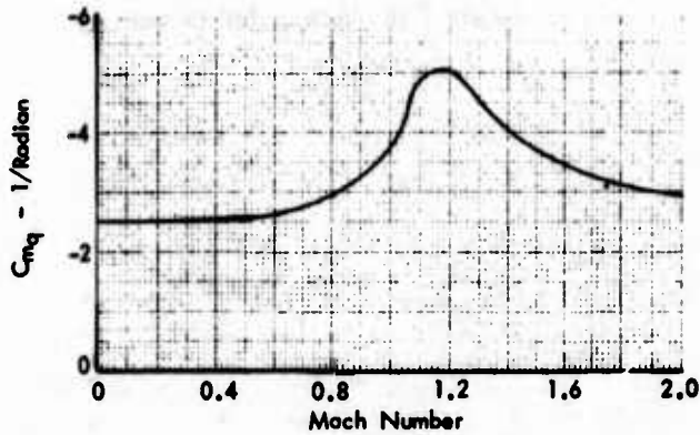
Figure I-11 Pitch Rate Derivatives
