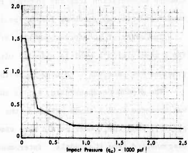
Figure I-23 Longitudinal Forward Loop Gain
