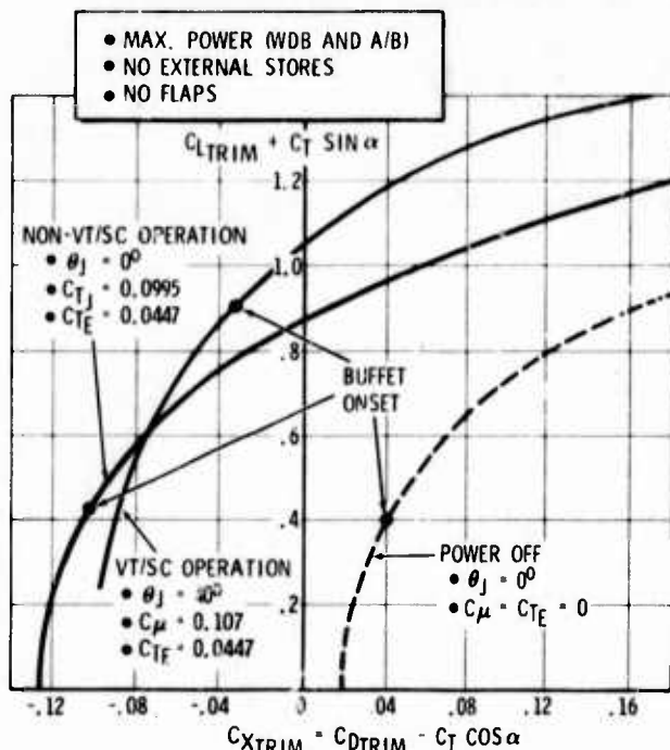
Figure 2-2 Typical LWA Aerodynamic Performance at MO. 9, 30,000 Feet Altitude
