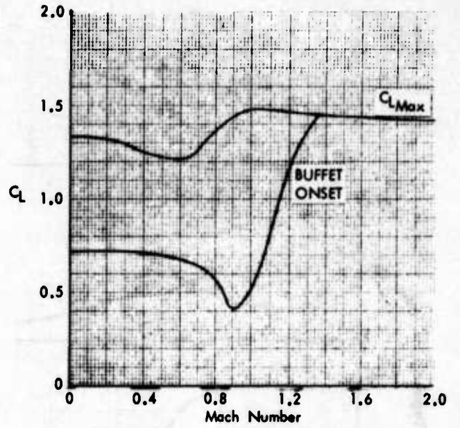
Figure I-12 Maximum Lift Coefficient
