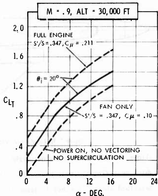
Figure B-32 Fan-Air-Only VT/SC Aerodynamic Performance Potential
