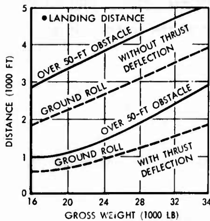
Figure A-1 Vectored Thrust Can Decrease Landing Distance and Increase Turn Rate
