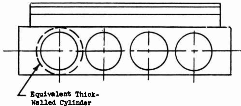
Figure 30. Manifold Dimension.
