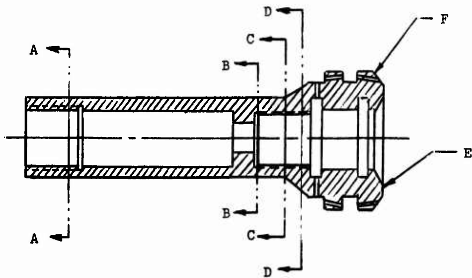
Figure 12. First-Stage Piston.
