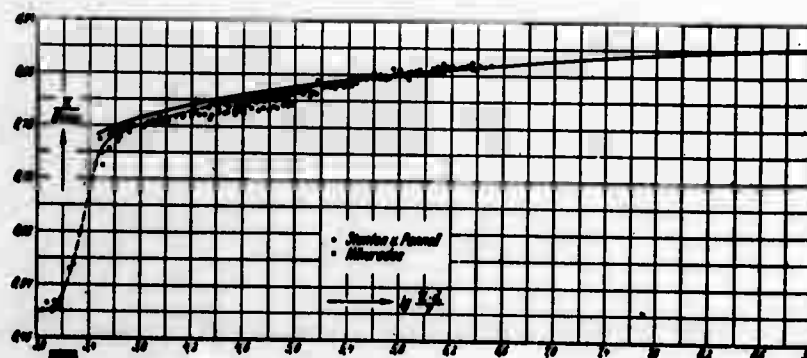
Fig. 39. \frac{U}{U_{max}} in Relation to \log\left(\frac{U d}{\nu}\right)
