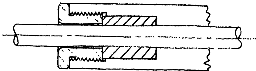
PRESSURIZED GROMMET
