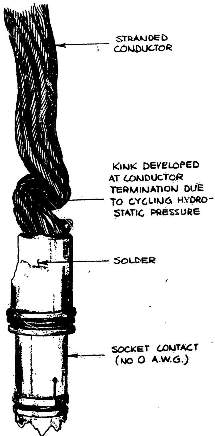
Figure 3-12. Typical Conductor Damage Due To Cycling Hydrostatic Pressure
