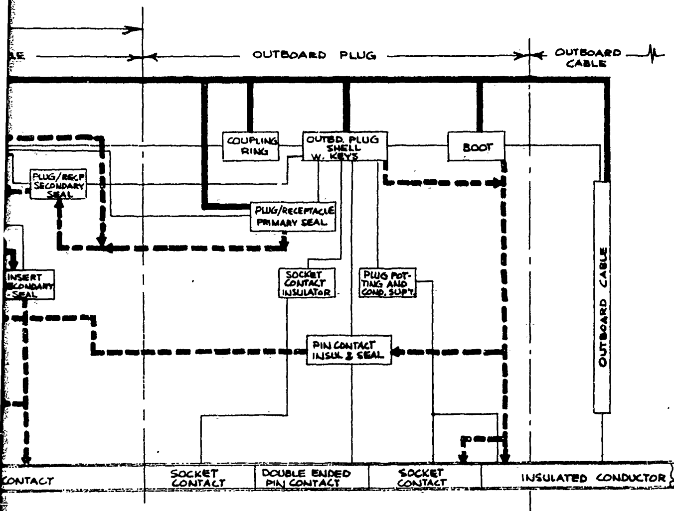
Figure 6-19. Detail Logic Block Diagram -
