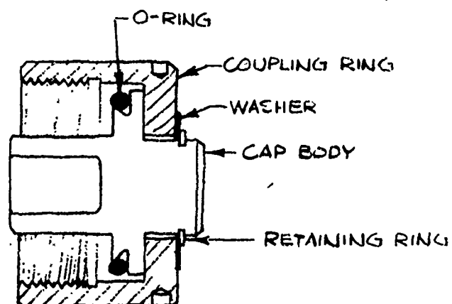
PRESSURE PROOF RECEPTACLE CAP
