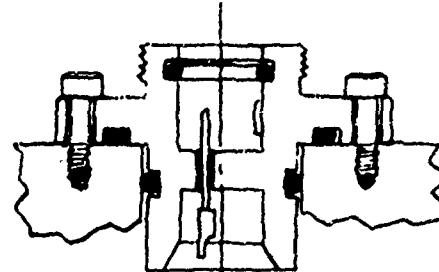
FLANGE BOLTED STYLE
