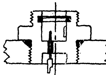
THREADED STYLE
