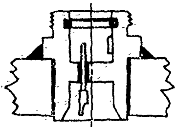
FLANGE WELDED STYLE
