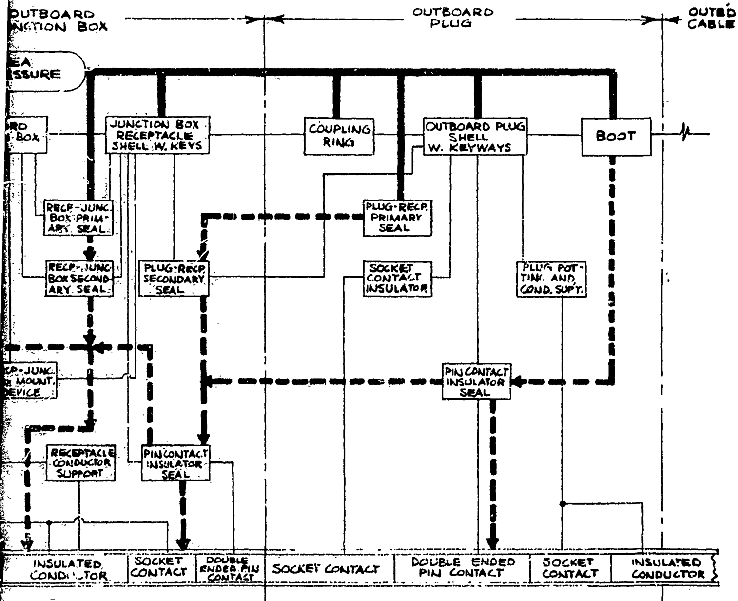
Figure 6-21. Detail Logic Block Diagram - Outboard Junction Box
