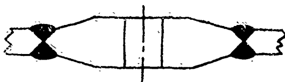
U.S. NAVY TYPE
