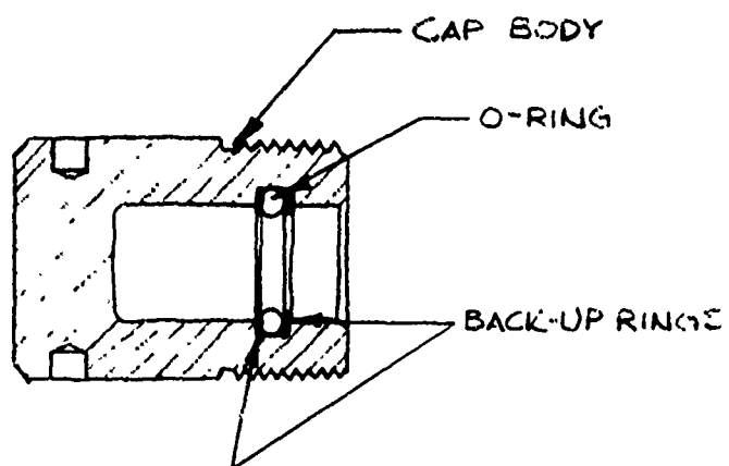
PRESSURE PROOF PLUG CAP
