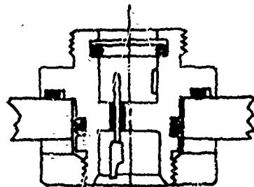
FLANGE/LOCKNUT STYLE
