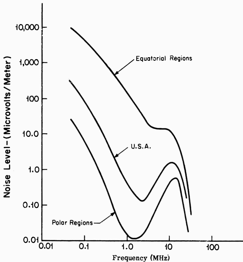
FIG. 1-1: Average Atmosphere Noise Level in Microvolts/Meter, as a Function of Frequency.
