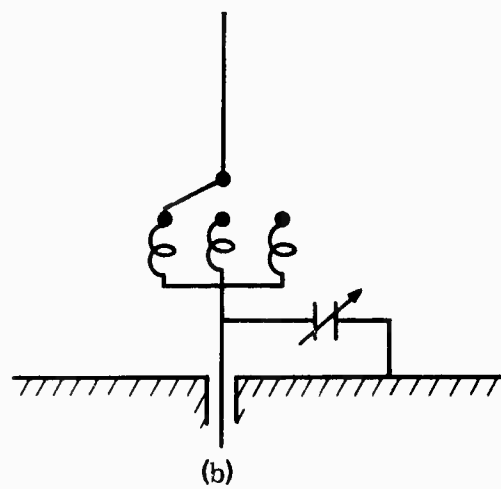
FIG. 3-9: Two Suggested Methods for Tuning and Matching Small Antennas with Highly Capacitive Input Impedance.
