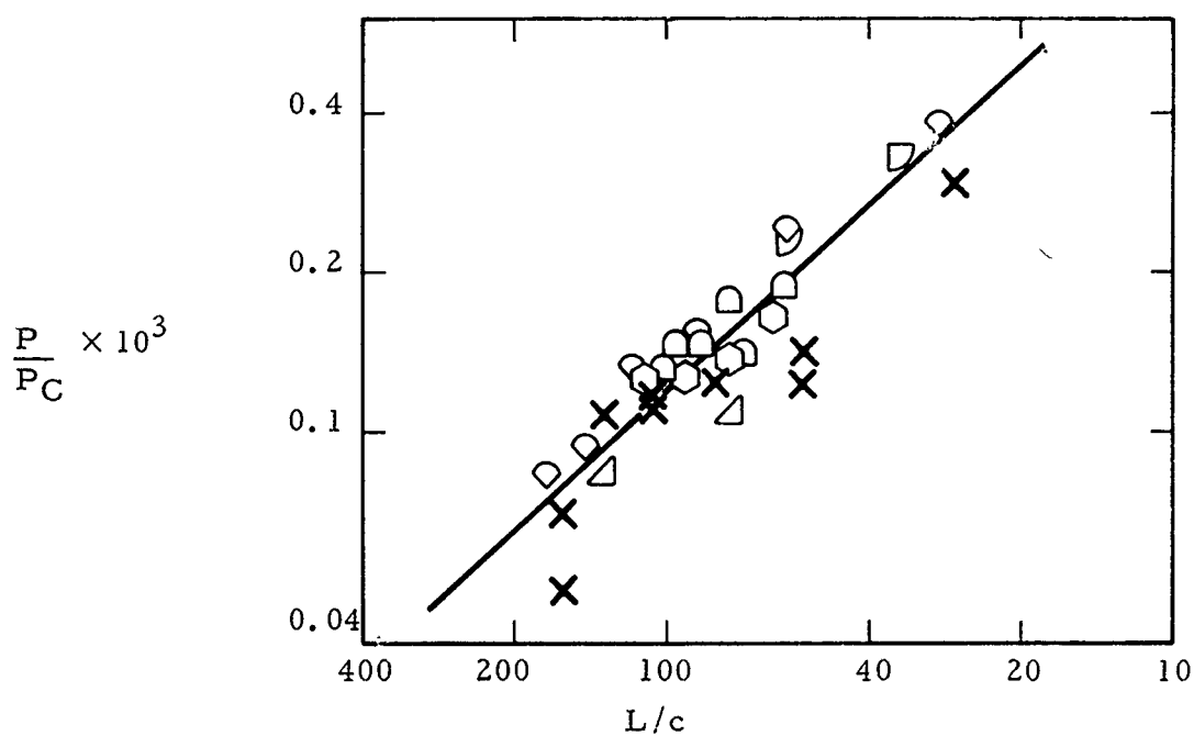
Fig. 26 Scaled Overpressures for Recoilless Rifles 90° to Breech
