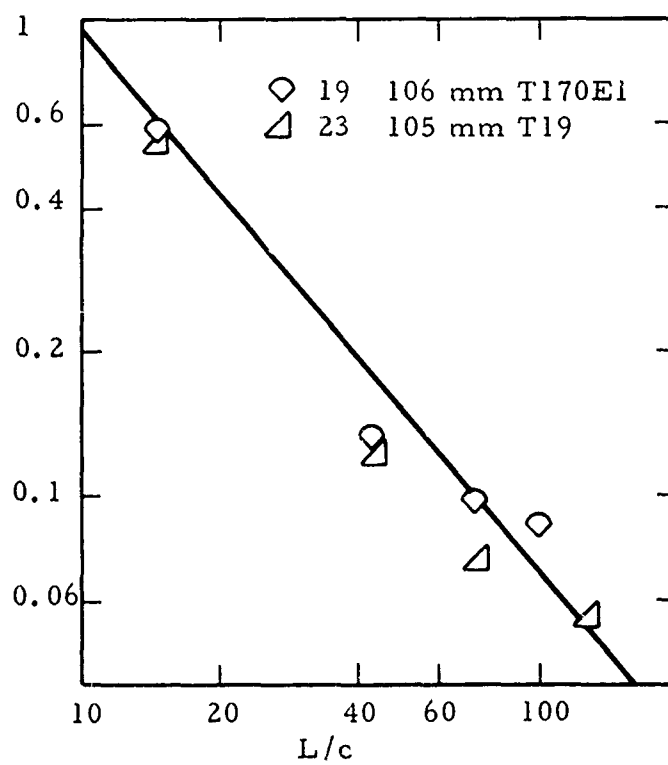
Fig. 32 Pressure 30° from Muzzle
