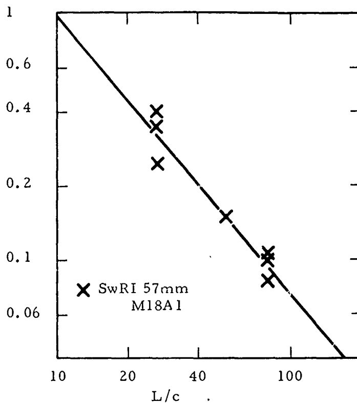
Fig. 31 Pressure 5° from Muzzle
