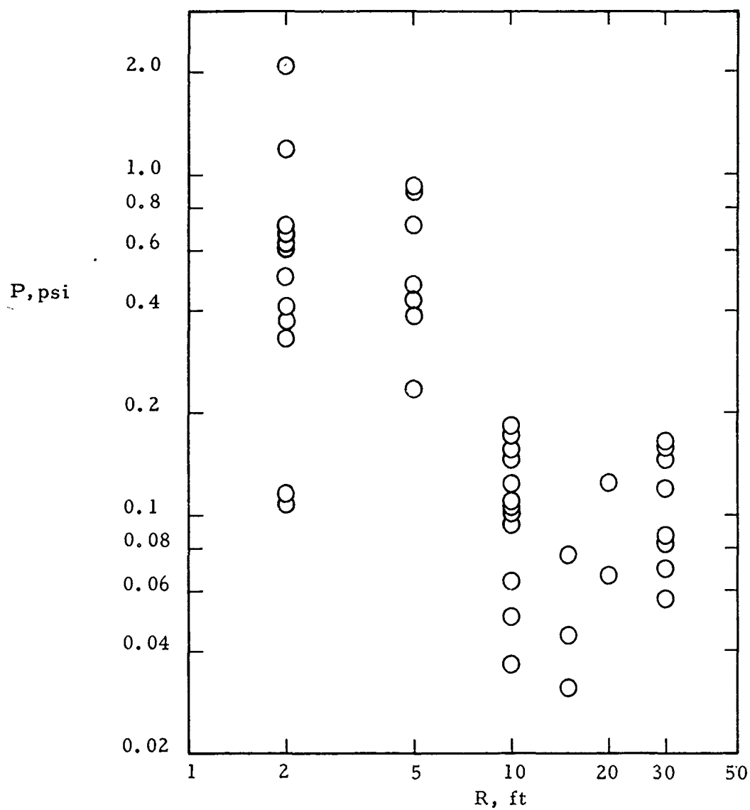
Fig. 15 Free-Field Overpressures vs. Distance 2.75 in Rocket, \theta = 135^\circ or 225^\circ
