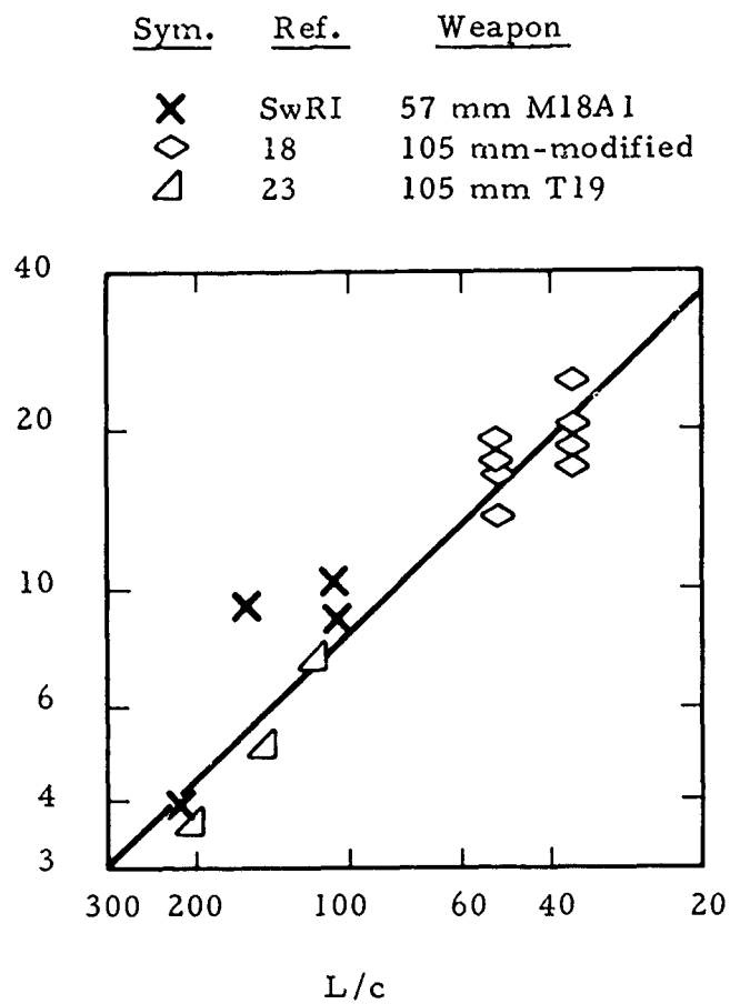
Fig. 28 Scaled Impulse for Recoilless Rifles, 0° to Breech
