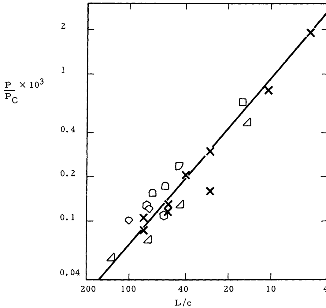
Fig. 27 Scaled Overpressures for Recoilless Rifles, 90° to Muzzle
