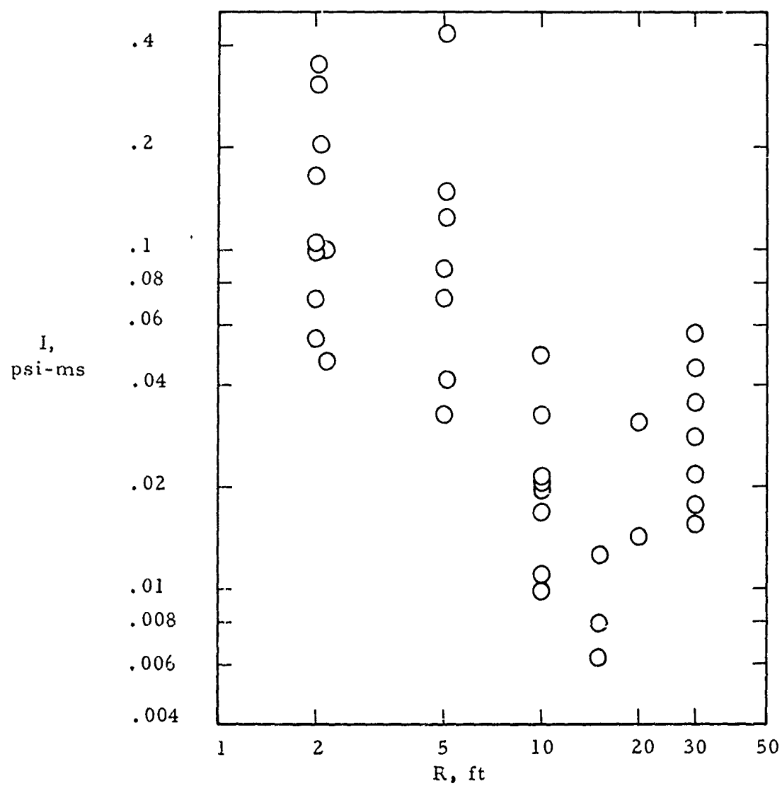
Fig. 16 Free-Field Impulse vs. Distance, 2.75 in Rocket, \theta = 135^\circ or 225^\circ
