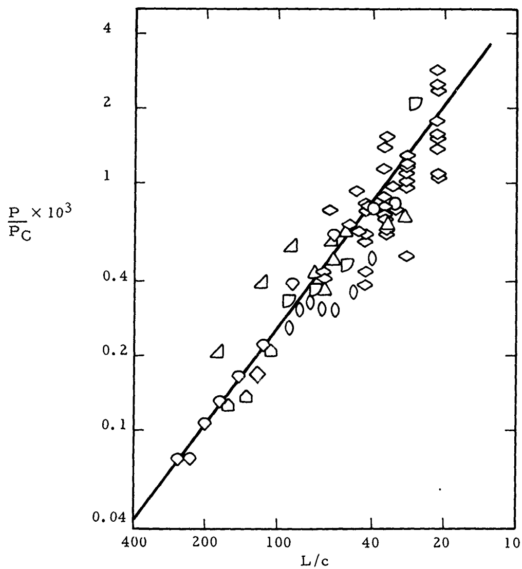
Fig. 25 Scaled Overpressure for Recoilless Rifles, 30° to Breech
