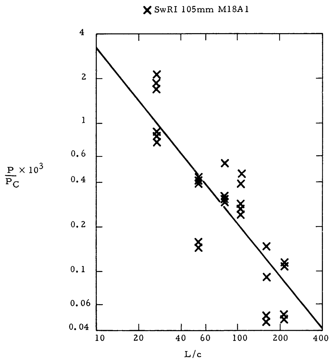
Fig. 37 Pressure at 45° from Breech
