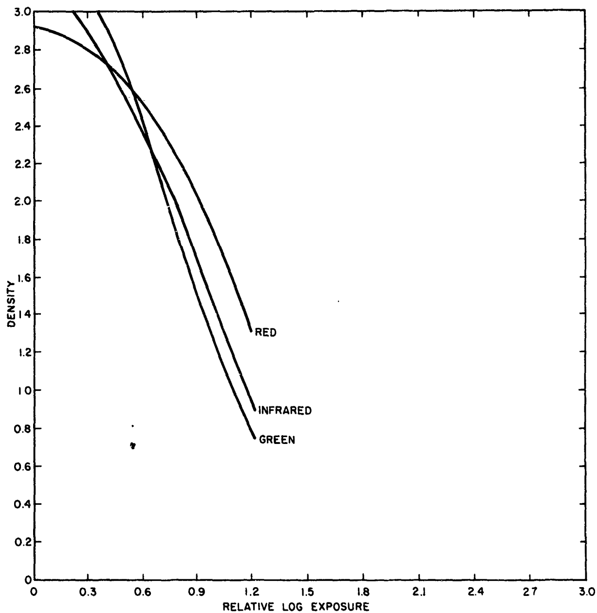
Figure 23. Response of Cyan Target Patch on Ektachrome Infrared Aero Film
