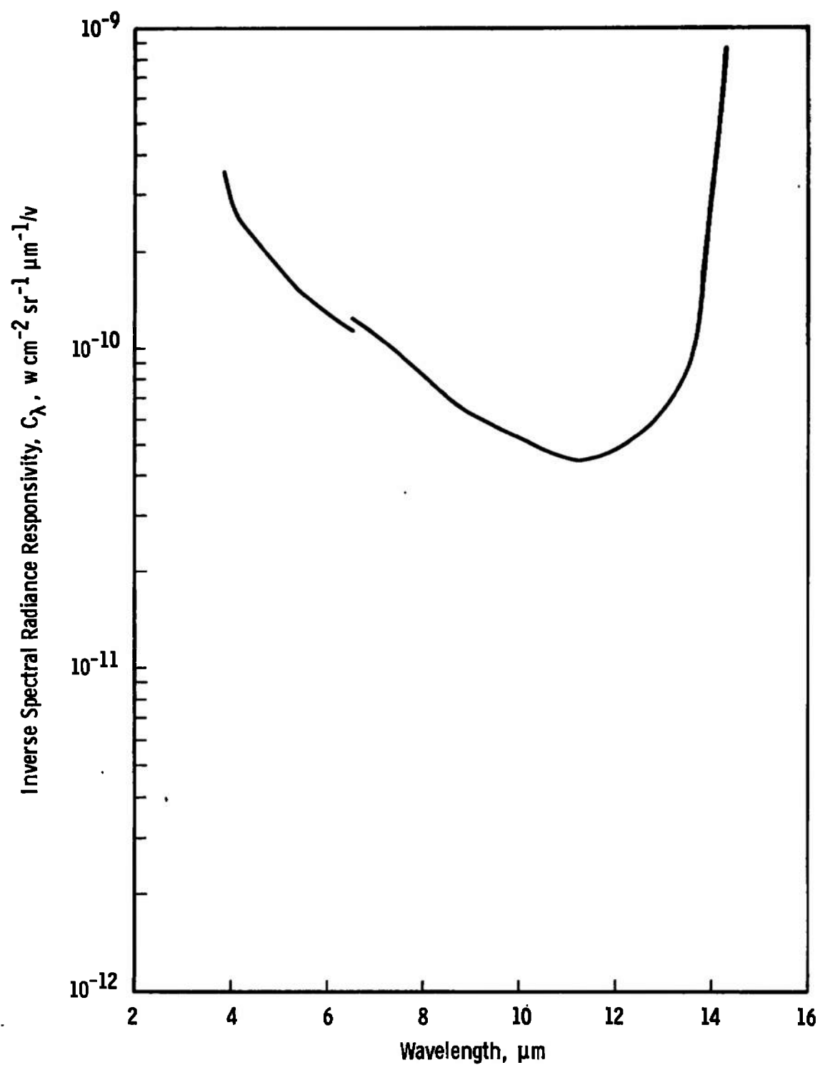
Fig. 10 HS-1 Inverse Spectral Radiance Responsivity
