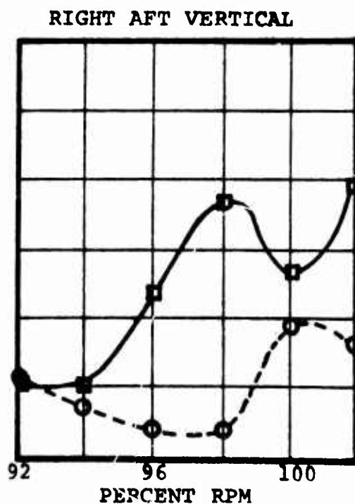
Figure 31. 105-Knot Four-Per-Rev Results of the 200-Pound With a Three-Inch CG Offset Unidirectional DAVI Platform on the Overload Gross Weight Helicopter.
