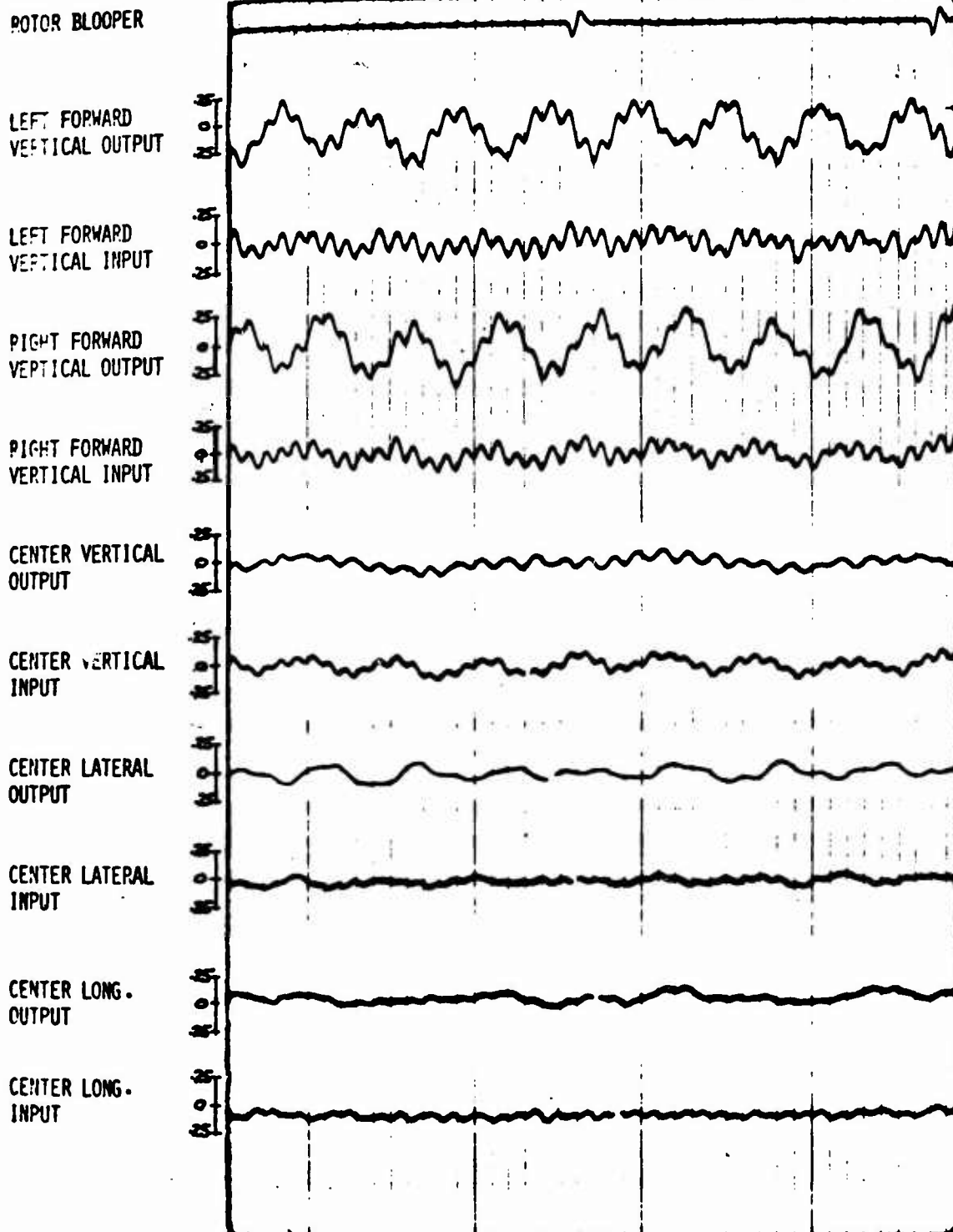
Figure 90. Oscilloscope Traces of the Level Flight Conditions for the 150-Pound Two-Dimensional DAVI Platform With Laterally Offset Pivots.
