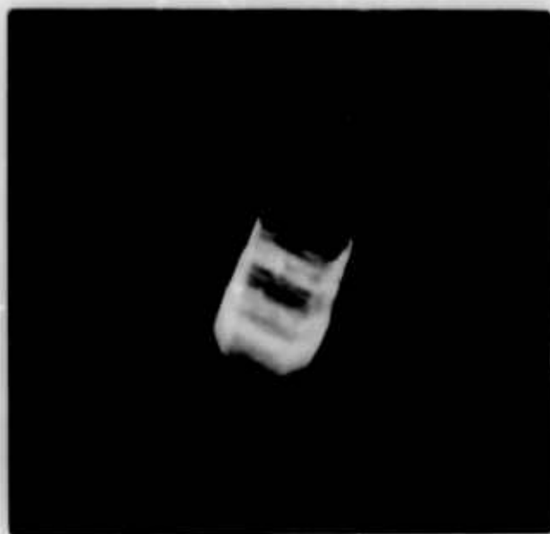
Figure 5. Scanning Electron Micrograph of Single W Fiber. Chemical Etch Has Altered Octagonal Cross Section at Fiber Base to a Square Shape at the tip. Pulsative Mode of SEM. X22,000
