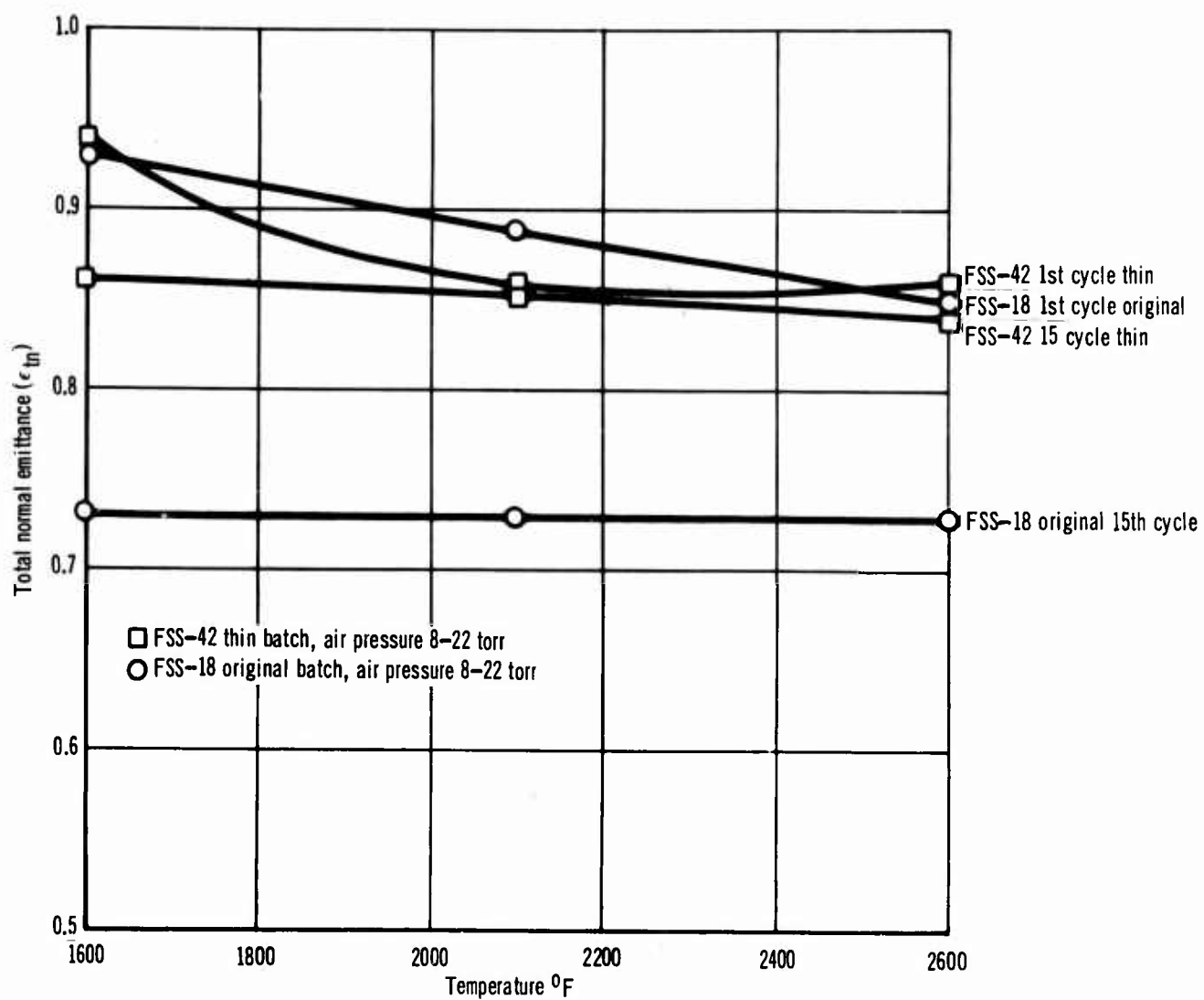
Figure 125 Emittance Of R-512E Coated Columbium (Original & Thin Batch) Versus Temperature (2600°F Max.)
