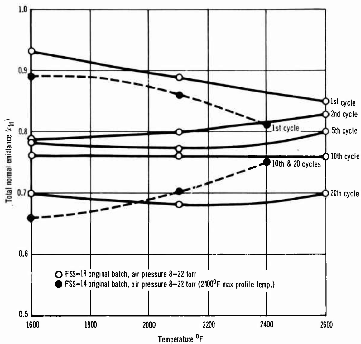
Figure 107 Emittance of R-512E Coated Columbium (Original Batch) Versus Temperature (2600°F Max)
