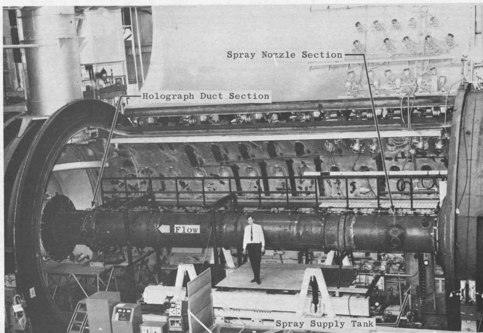
Figure 10. Test Installation
