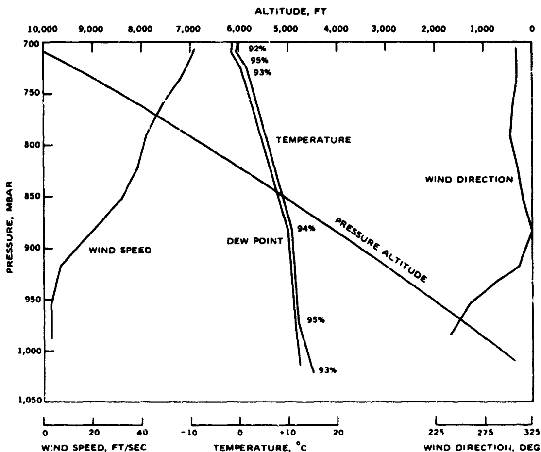
FIG. 32. Rawinsonde Data, Test 71.
