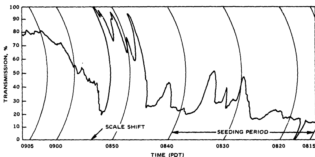
FIG. 25. Transmissometer Data, TF Right, Test 65.
