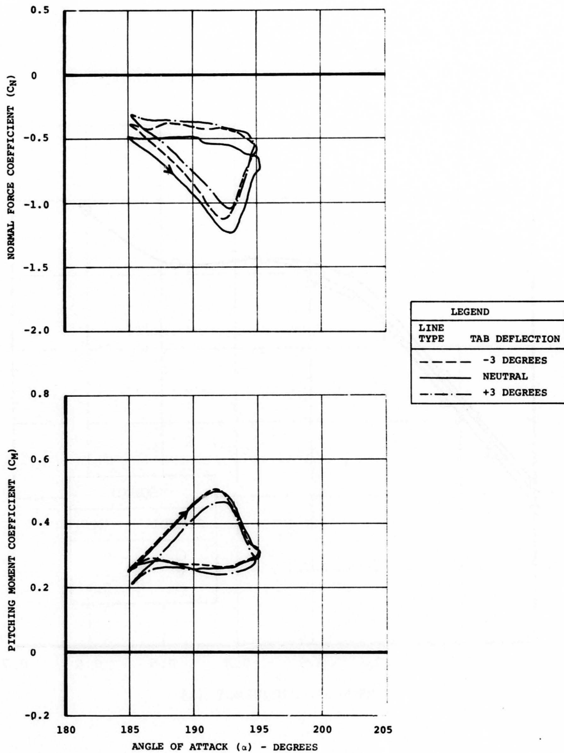
Figure 12. Effect of Trailing-Edge Tab Deflection on Dynamic C_N and C_M Versus \alpha at M = 0.3 and f = 16 Hertz.
