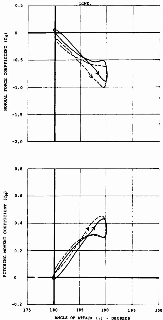
Figure 6. Comparison of Dynamic C_N and C_M Versus \alpha for Pitch Oscillation at f = 16 Hertz, M = 0.2 , \Delta\alpha = 5 Degrees, and for Mean Angles of Attack Greater Than and Less Than 180 Degrees.
