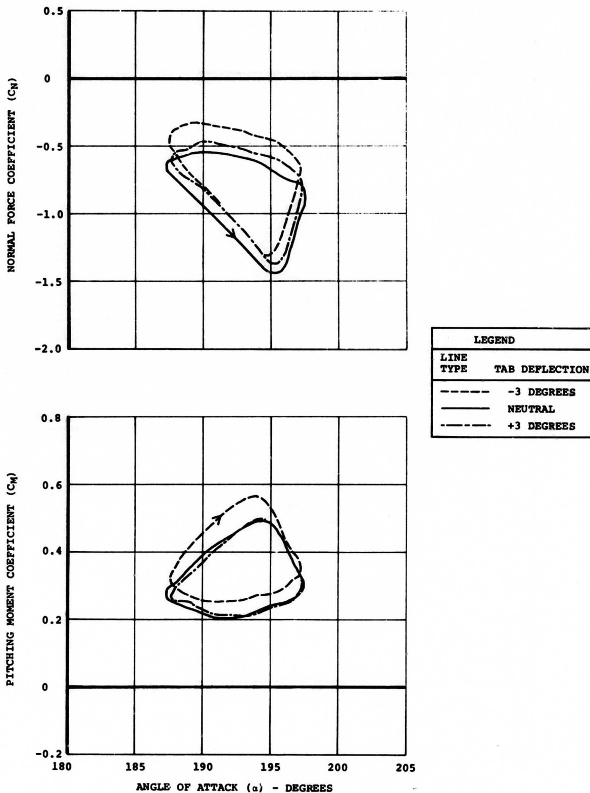
Figure 10. Effect of Trailing-Edge Tab Deflection on C_N and C_M Versus \alpha at M = 0.2 , f = 16 Hertz, and \alpha_0 = 192.5 Degrees.
