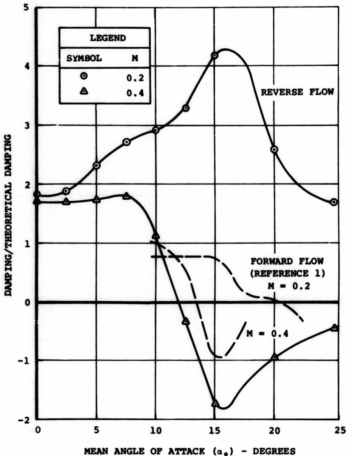
Figure 32. Comparison of Aerodynamic Pitch Damping for Forward and Reverse Flow at f = 96 Hertz, \Delta\alpha = 2.5 Degrees.
