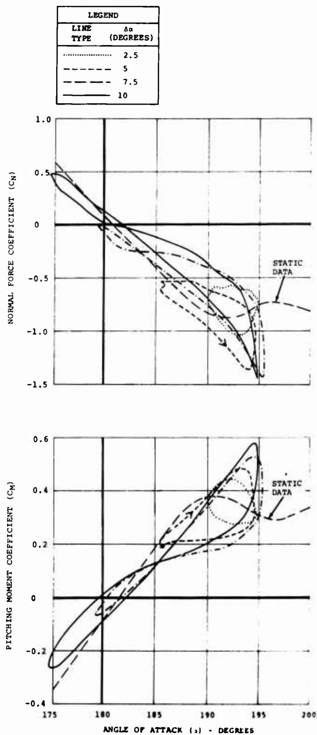
Figure 8. Effect of Oscillation Amplitude on Dynamic C_N and C_M Versus \alpha for Pitch Oscillation at f = 16 Hertz, M = 0.2 , and Constant Maximum \alpha .
