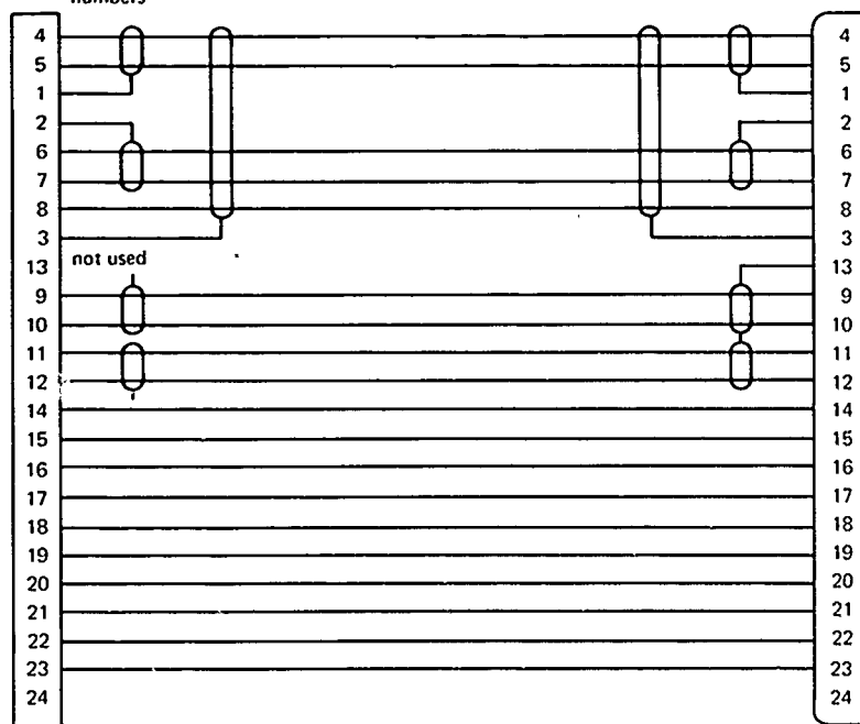
Figure 2. Umbilical schematic (primary).
