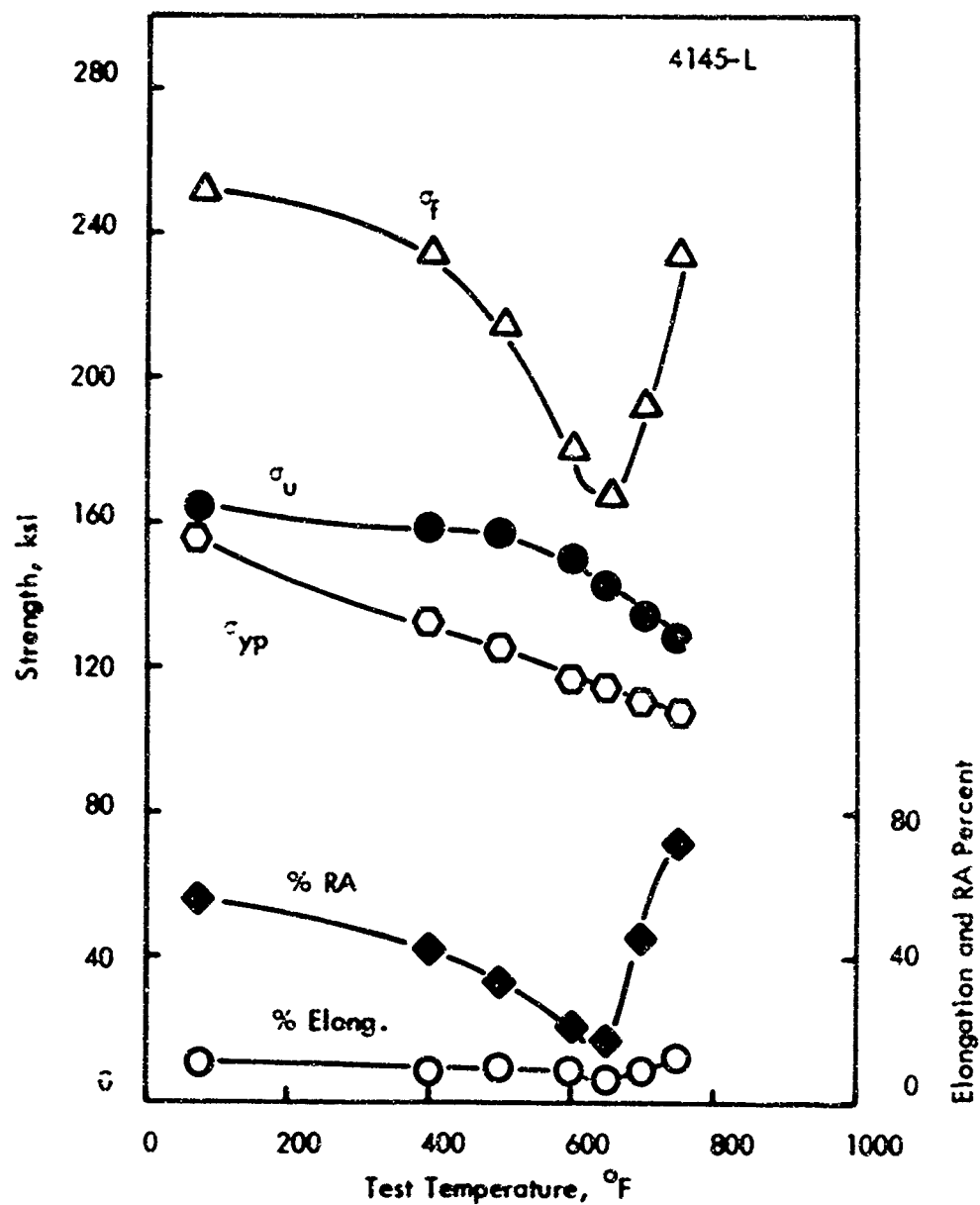
Fig. 51. Elevated Temperature Tensile Properties of Internally Landed 4145 Steel Heat Treated to the Prior Deformation Strength Level (160 ksi) Used in the 30% Cold Working by Die Drawing Process.
