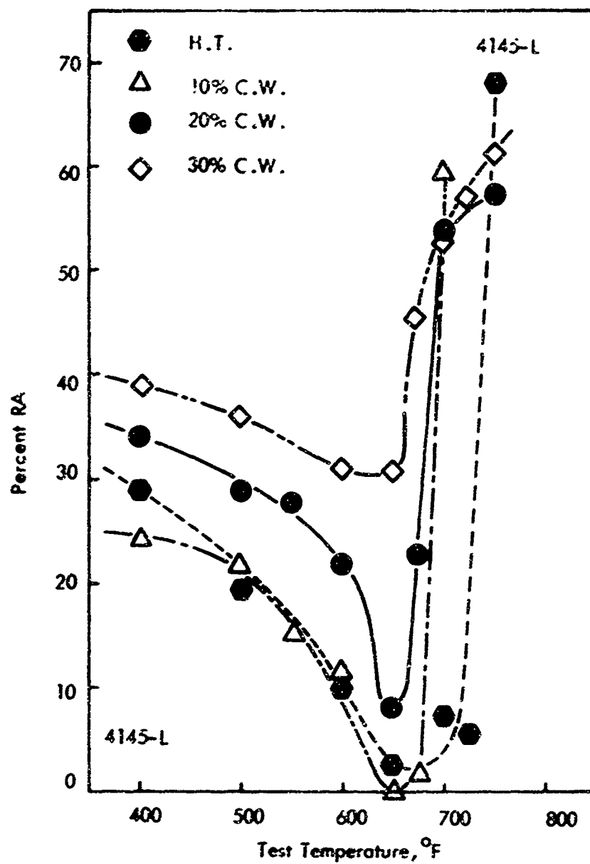
Fig. 59. Comparison of Ductility Properties of Internally Led 4145 Steel Processed to 200 ksi Nominal UTS by Heat Treatment Alone and Heat Treatment Plus 10, 20 and 30% Reductions by Die Drawing.
