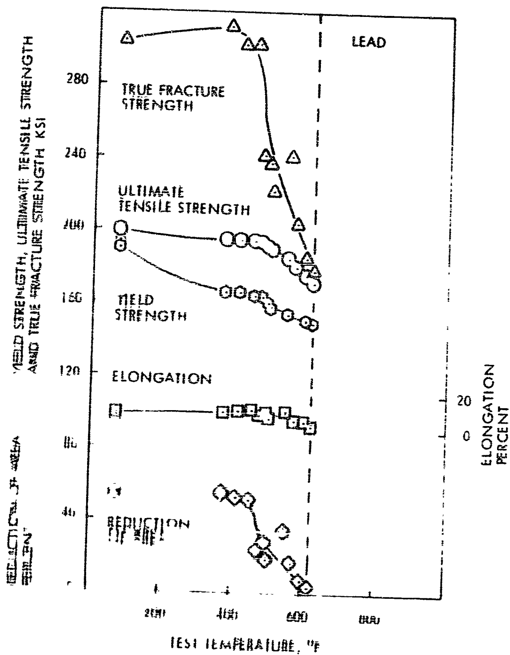
Fig. 2 Elevated Temperature Tensile Properties of 4140 Steel at 100 ksi Nominal Strength Level, and Surface Treated with P. & L. 195 9999-1
