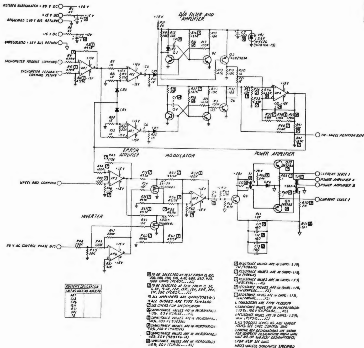
Figure 8. Wheel Control Electronics (Drawing 3064414)
