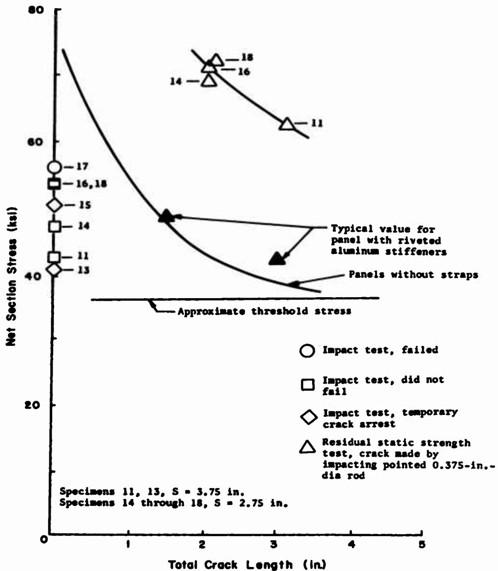
Figure 7. Crack Arrest and Residual Static Strength of 12-Inch by 0.032-Inch 7075-T6 Bare Panels, Two Straps on Front and Back Sides of Specimen.
