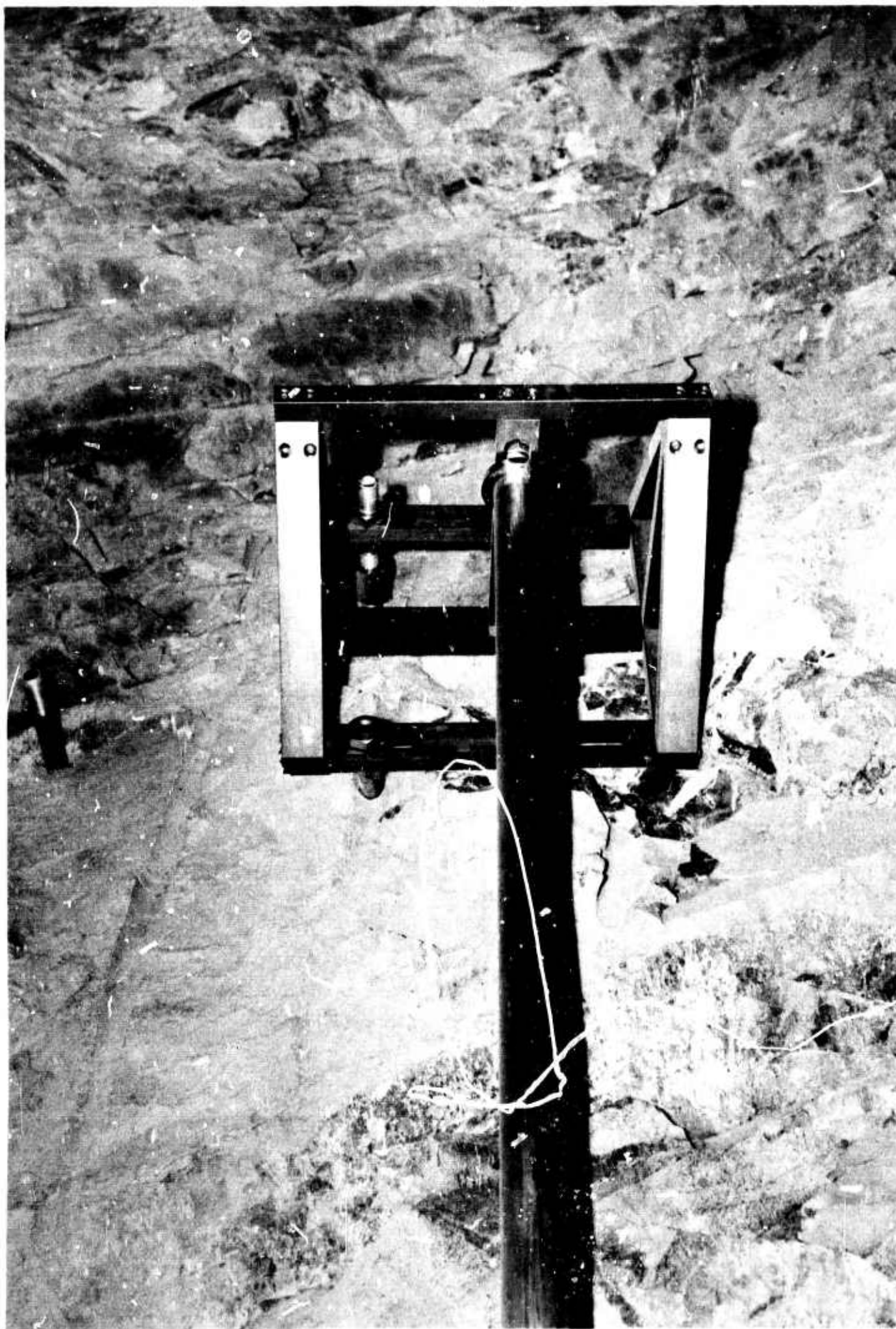
Figure 10. Strain rod anchor.
