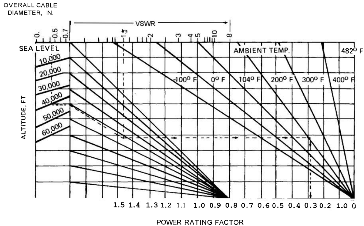
Figure 5-16. Power Rating Due to VSWR—Teflon Cable
