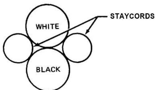
Figure 9-1. Special Purpose Cable—WD 27 A/U
