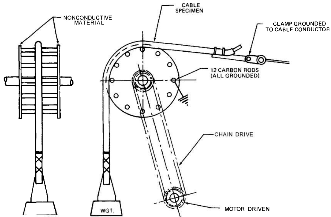
Figure 6— 15. Tungsten Carbide Rod Abrasion Test Apparatus
