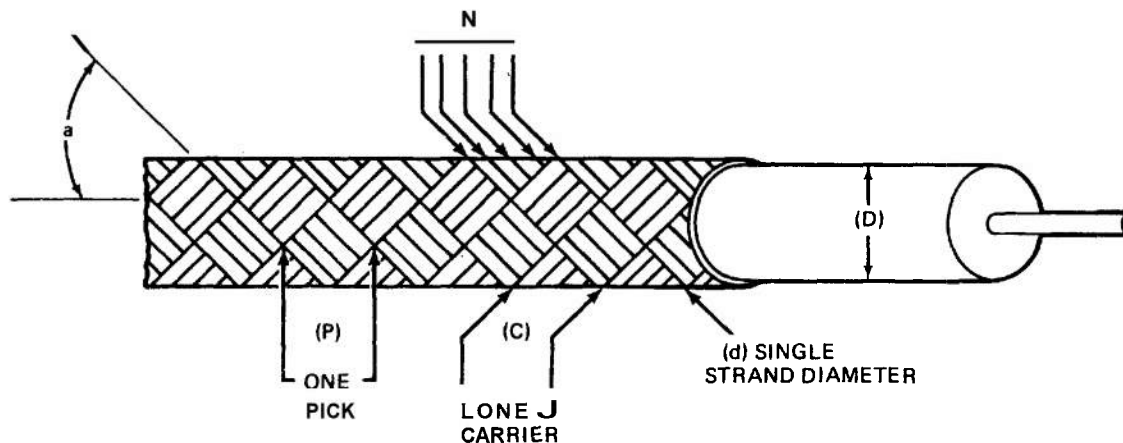
Figure 1-1. Shield-Constructional Details
