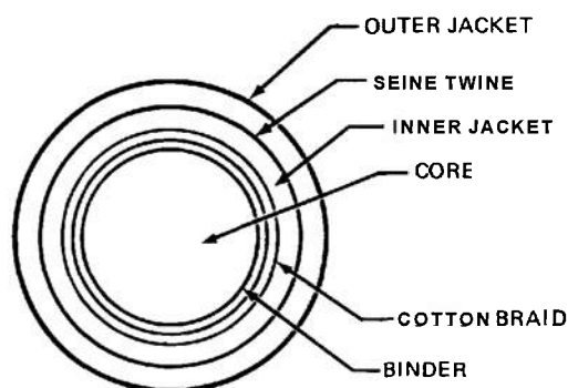
Figure 6-6. Reinforced Sheath Configuration
