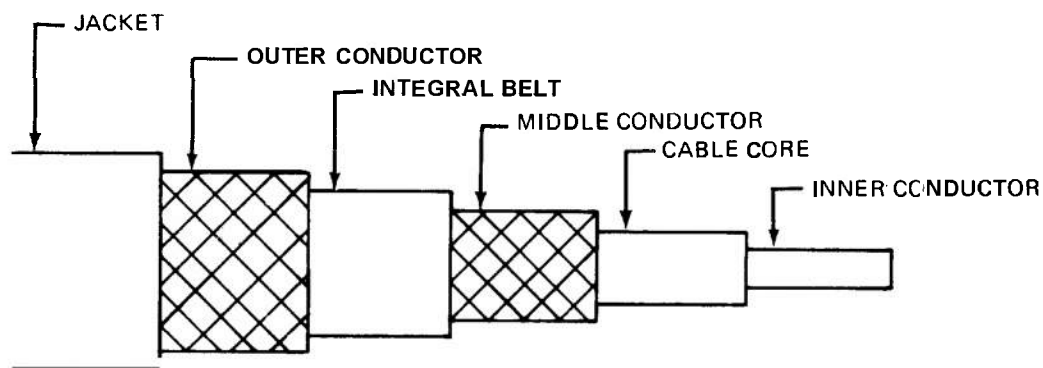
Figure 5-7. Triaxial Cable
