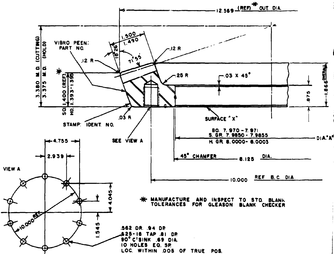
Figure 53. Gear Drawing for 7-1/2-Inch Cutter Diameter Test Gear Set.
