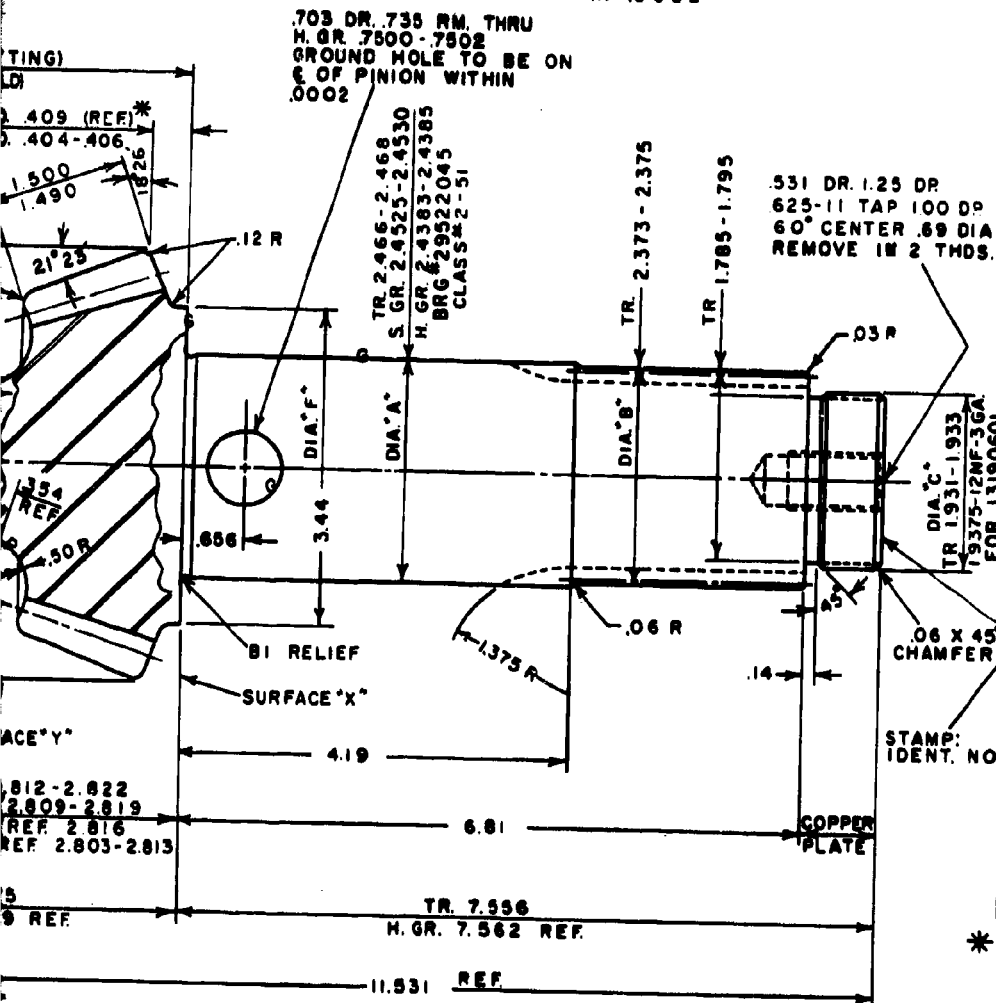
2. Pinion Drawing for 12-Inch Cutter Diameter Pulser Gear Set.
