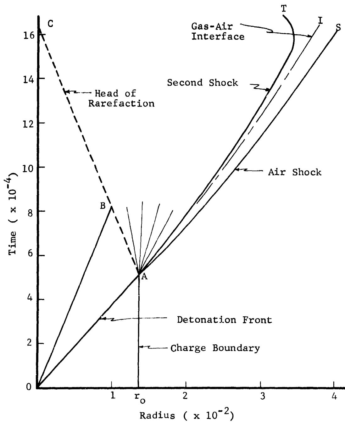
Figure 5 Early Expansion of Explosion Gas
