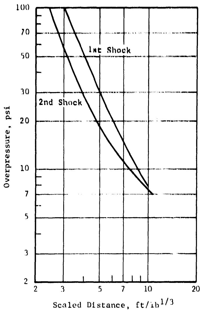
Figure 22 Pressures, Run No. 7, Charge Weight Ratio 2:1, Time Delay 1.10 \text{ms}/\text{lb}^{1/3}
