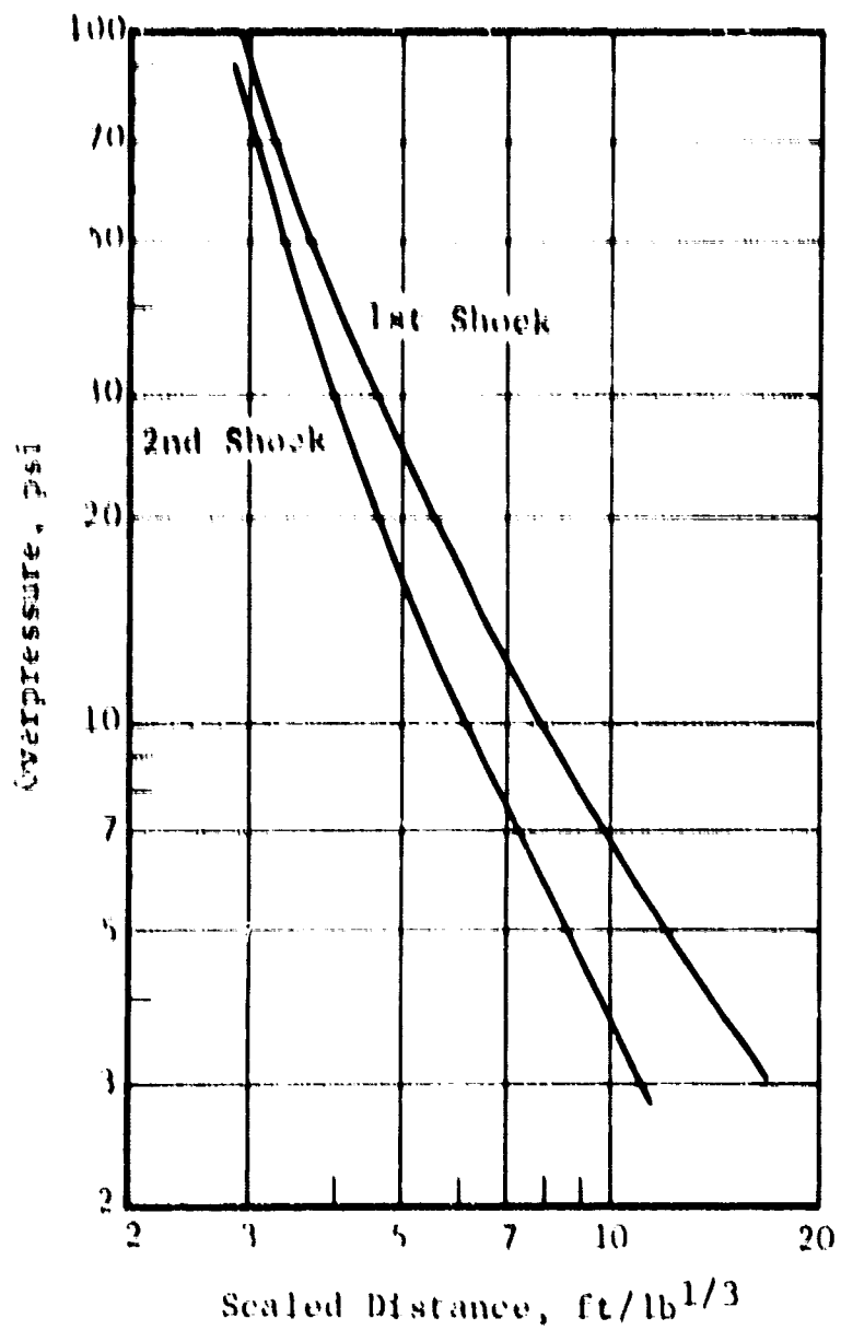
Figure 20 Pressures, Run No. 4, Charge Weight Ratio 1:1, Time Delay 4.18 \text{ms}/\text{lb}^{1/3}
