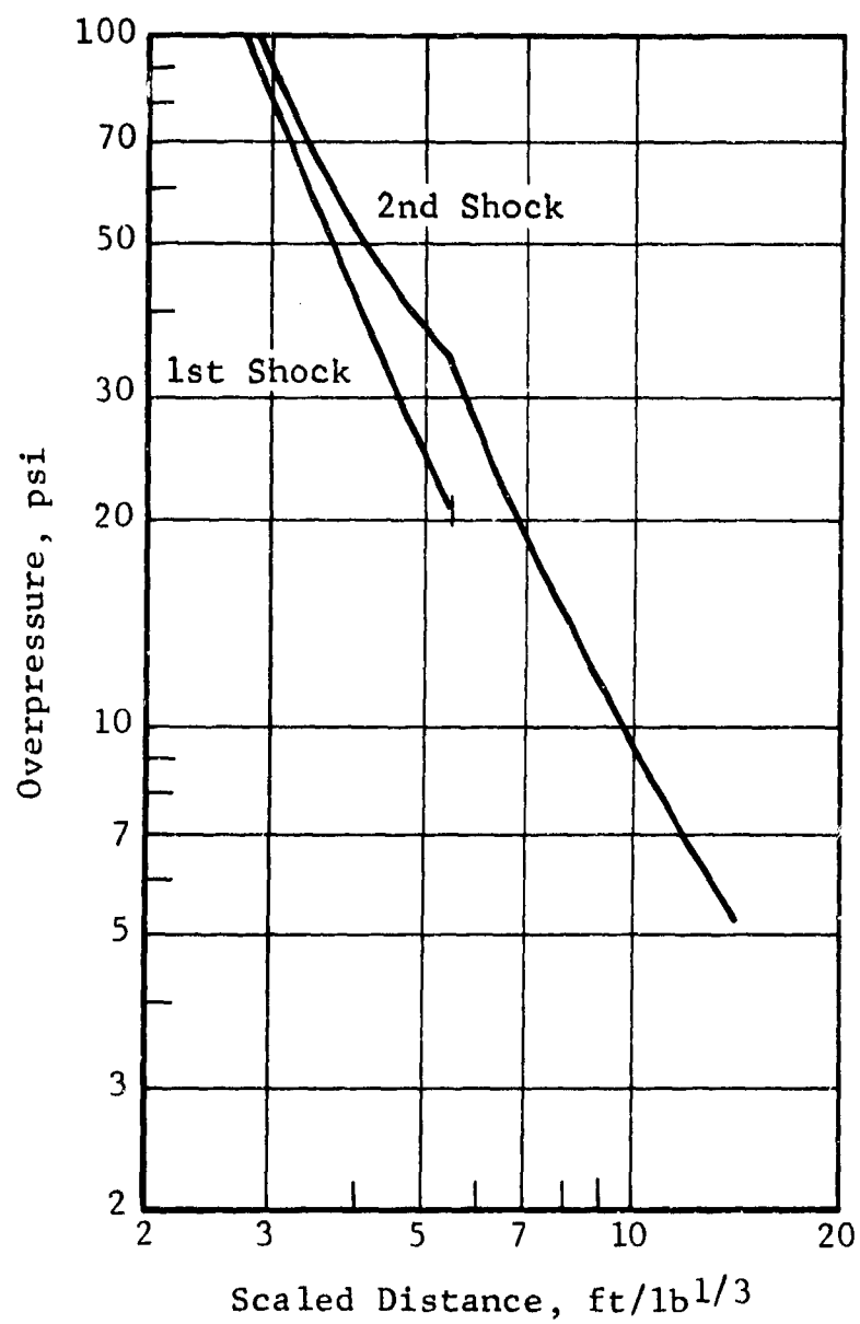
Figure 16 Pressures, Run No. 1, Charge Weight Ratio 1:1, Time Delay 0.59 ms/lb 1/3
