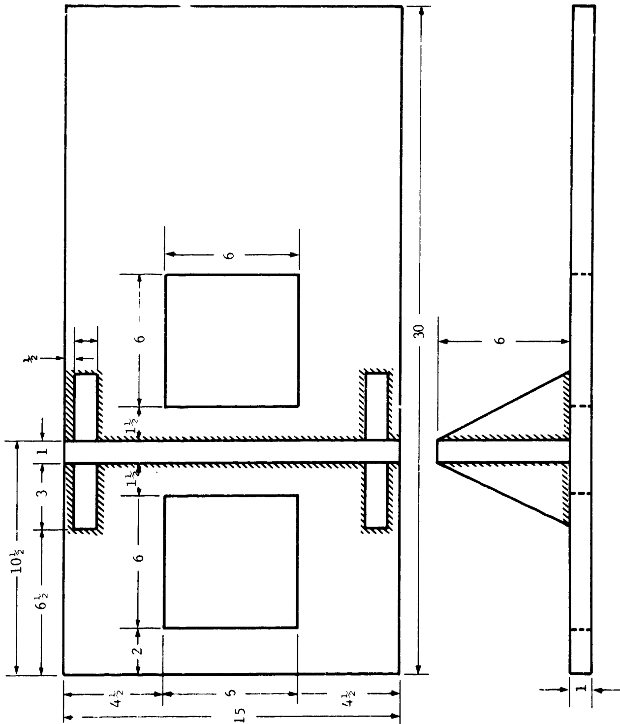
Figure 26 Test Fixture
