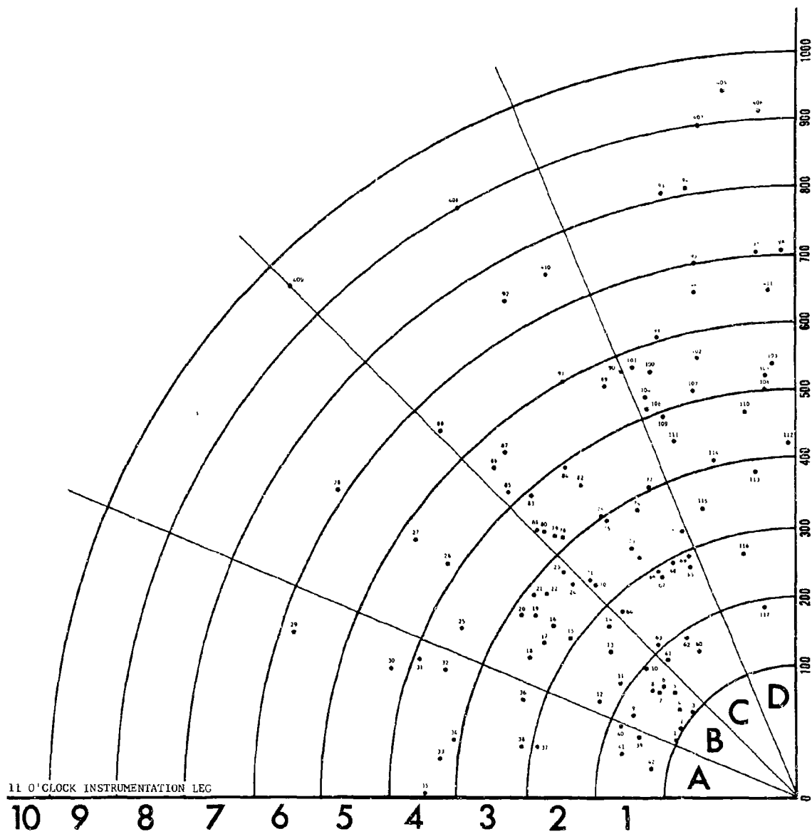
Fig. 3-1. S-IV Fragment Locations (Quadrant I)
