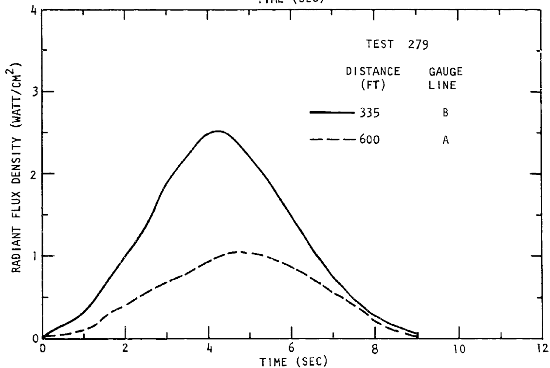
Fig. 2-37. Radiant Flux Density Outside the Fireball from Tests 277 and 279
