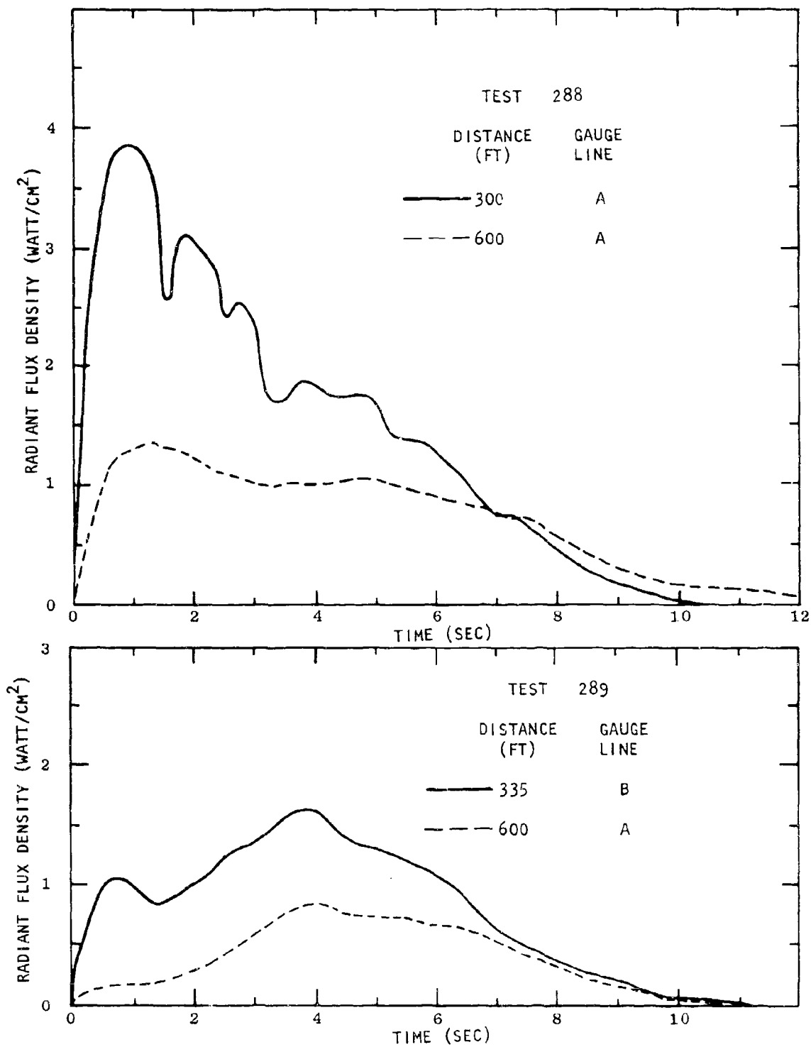
Fig. 2-38. Radiant Flux Density Outside the Fireball from Tests 288 and 289
