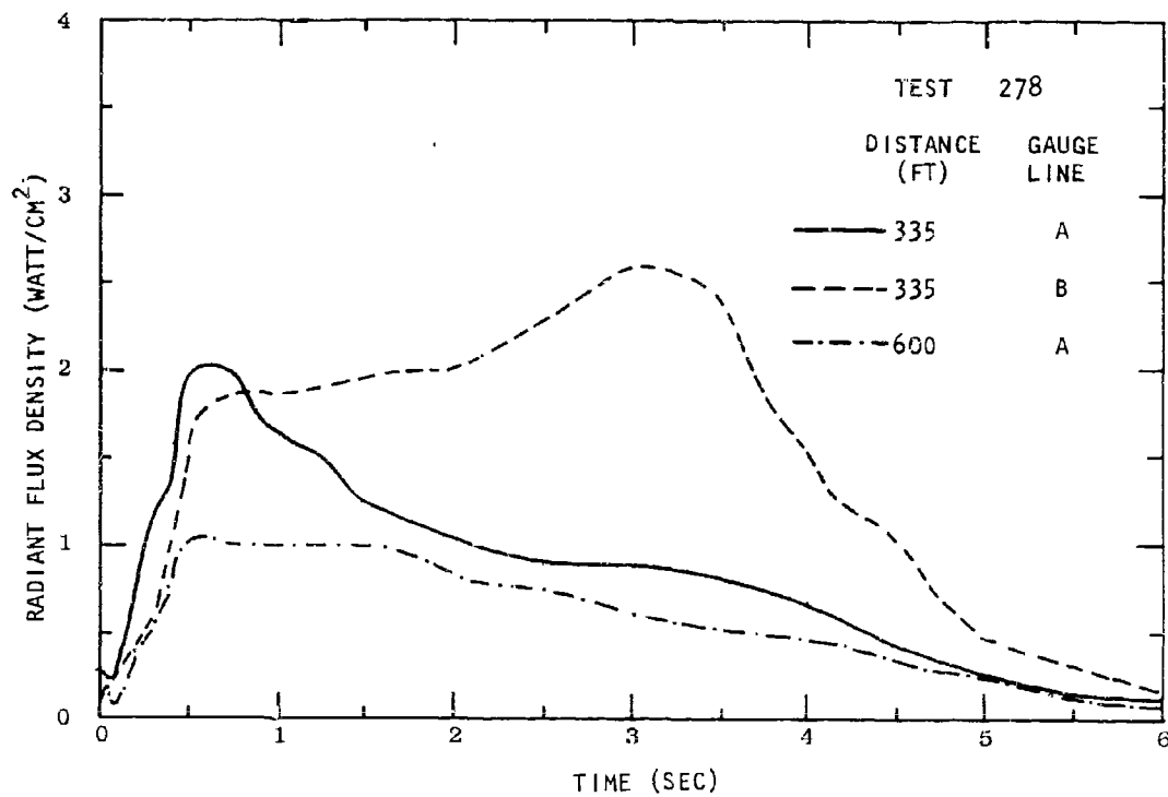
Fig. 2-34. Radiant Flux Density Outside the Fireball from Tests 275 and 278
