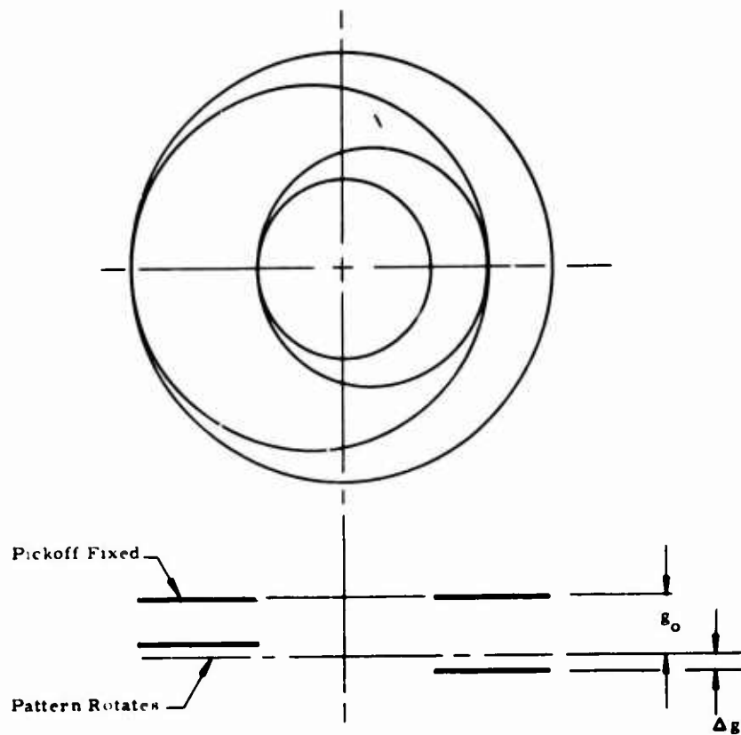
Figure 41. Gap Runout
