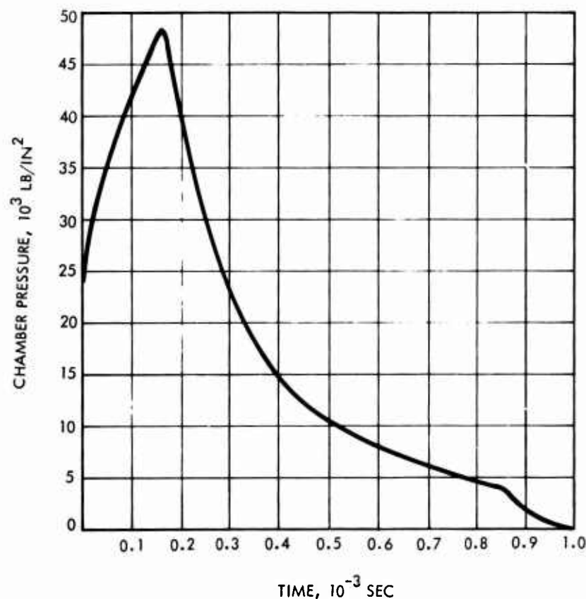
Figure I-1. HIVAP Gun Chamber Pressure Transient
