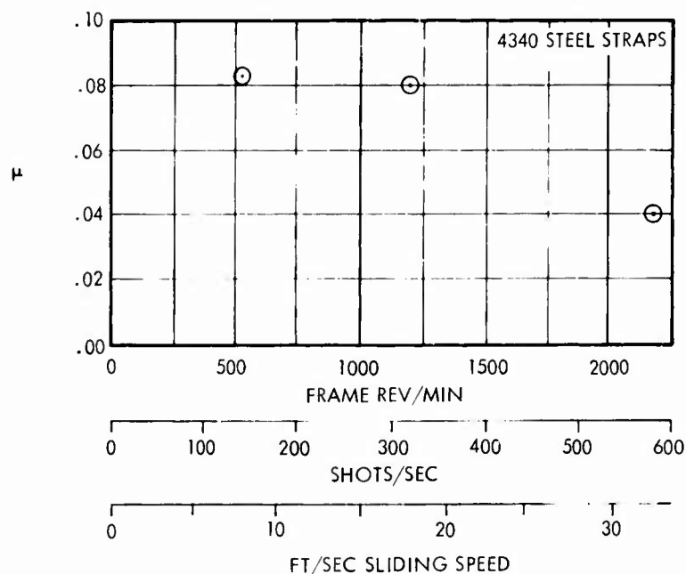
Figure 18. Friction Coefficient Versus Rate MoS 2 Lubricant
