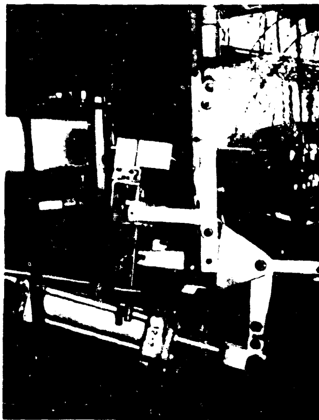
Figure 91 Closeup View of High-Temperature Material Cyclic Endurance Test Rig Showing Specimens in Test Position
