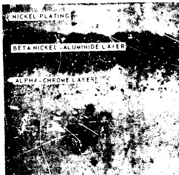
Unetched Mag: 1000X Figure 78 Photomicrograph of TD Nickel Specimen With Duplex Chrome-Aluminate Coating NOFORN
