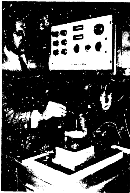
Figure 16 EDM Equipment Designed for Small-Diameter Hole Drilling
