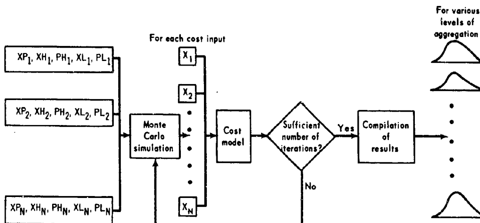
Fig. 8—Monte Carlo Technique, Weibull Variant
