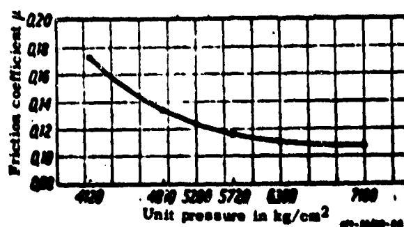
Fig. 8. Dependence of the coefficient of friction \mu of synthetic molybdenum disulphide on contact pressure for a constant sliding speed v = 482.6 m/min.
