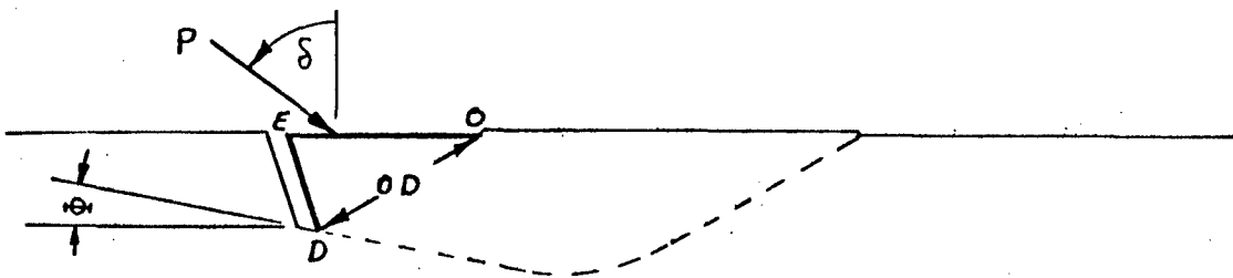
Figure 3. Configuration of plate and soil after a small plate displacement. Soil below the dashed curve has remained rigid.
