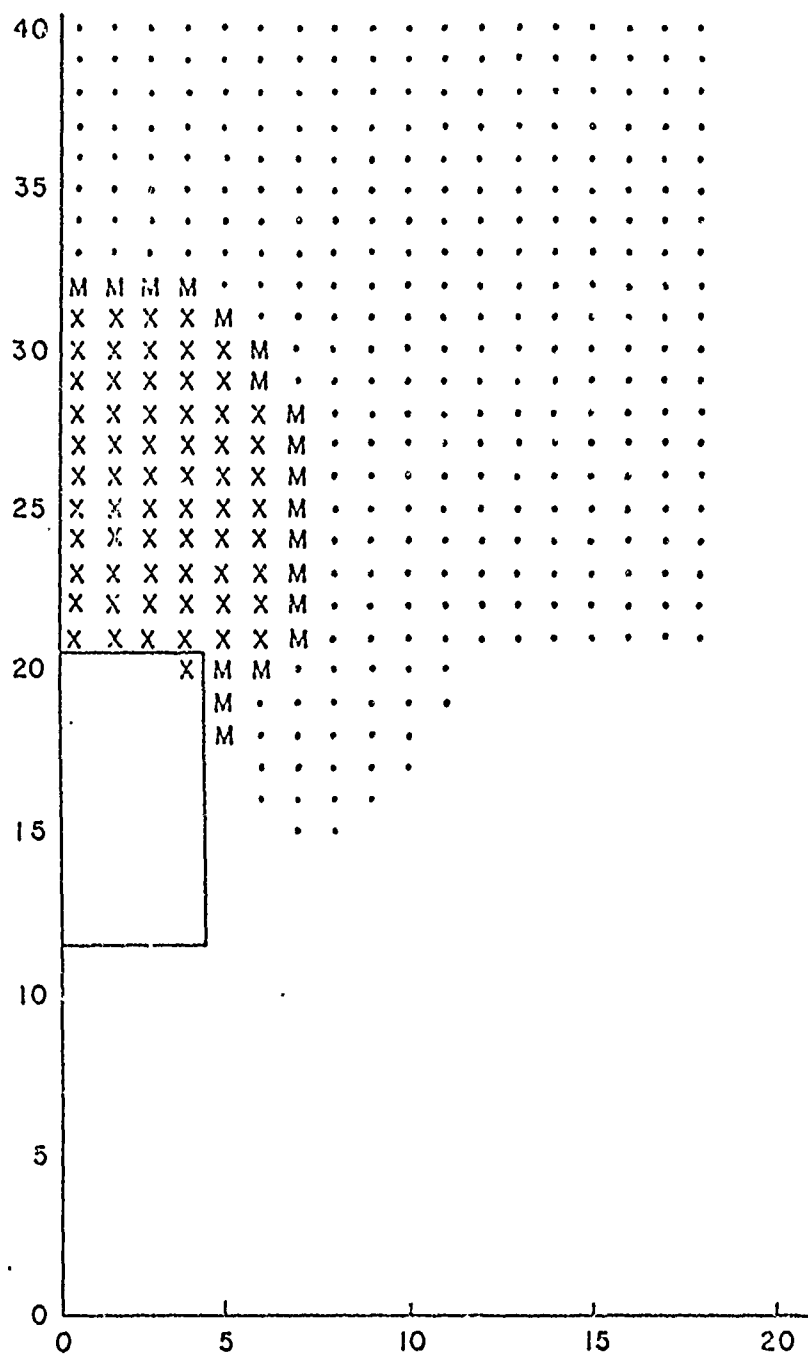
Fig. 2--Cell configuration for the TOIL code at a time of 16.1 \mu sec
