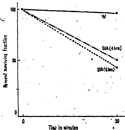
Fig. 2 Thermal inactivation of the SVA (after infection for 4 and 6 hours) and myxoma virus (MV) after incubation at 37°C for 30 minutes
