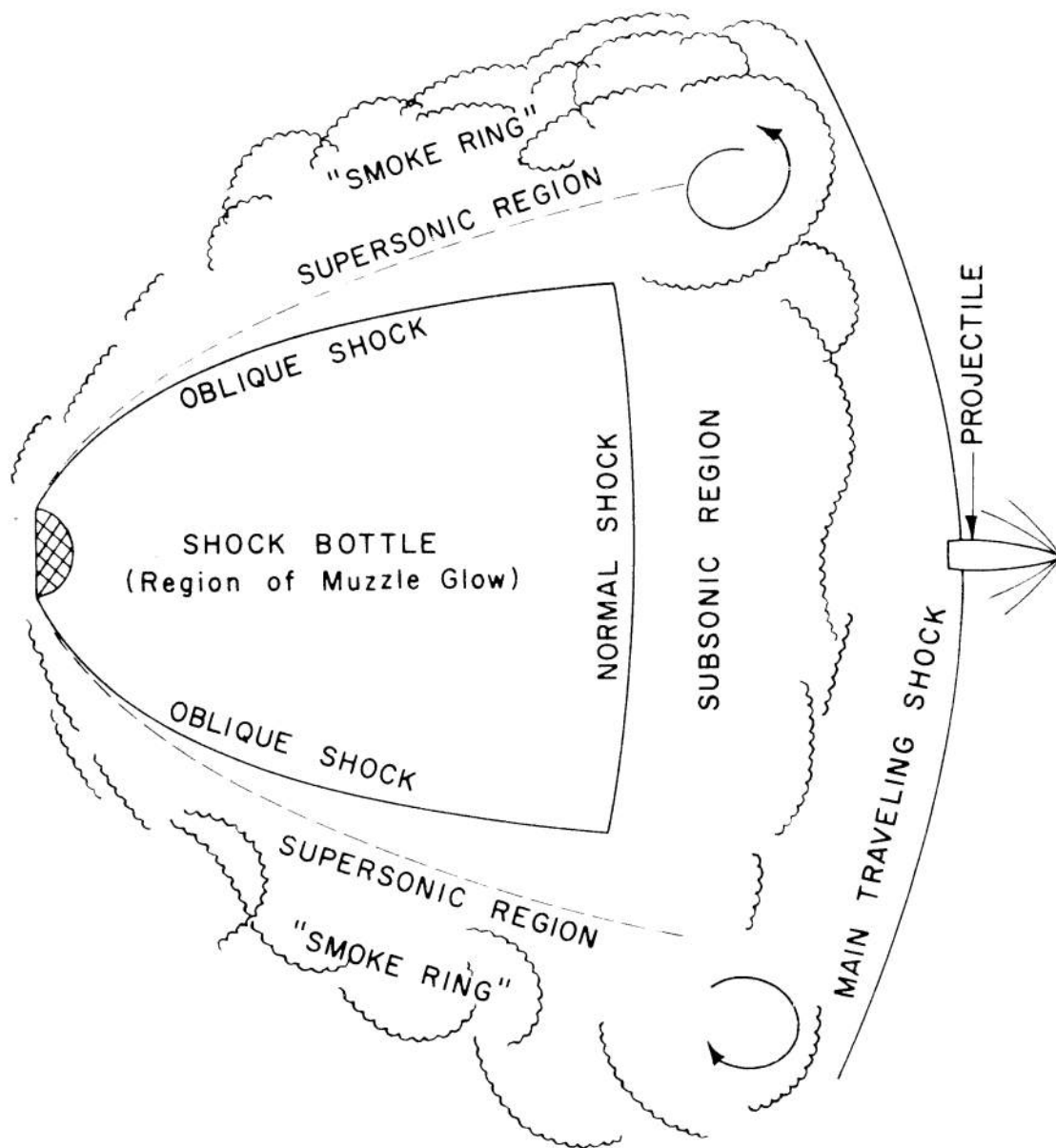
FIGURE 2-1. MAXIMUM VOLUME STAGE OF SHOCK BOTTLE
