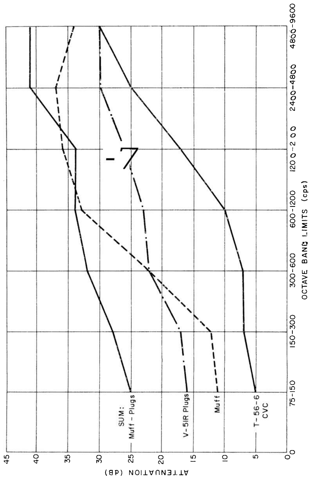
FIGURE 9-5. CHARACTERISTICS OF EAR PROTECTIVE DEVICES
