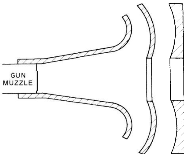
FIGURE 1—1. SCHEMATIC OF CLOSED MUZZLE BRAKE
