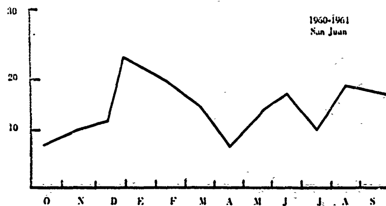
Fig. 6. Annual Monthly Average (Number of colonies per 12 minutes of daily exposure.)
