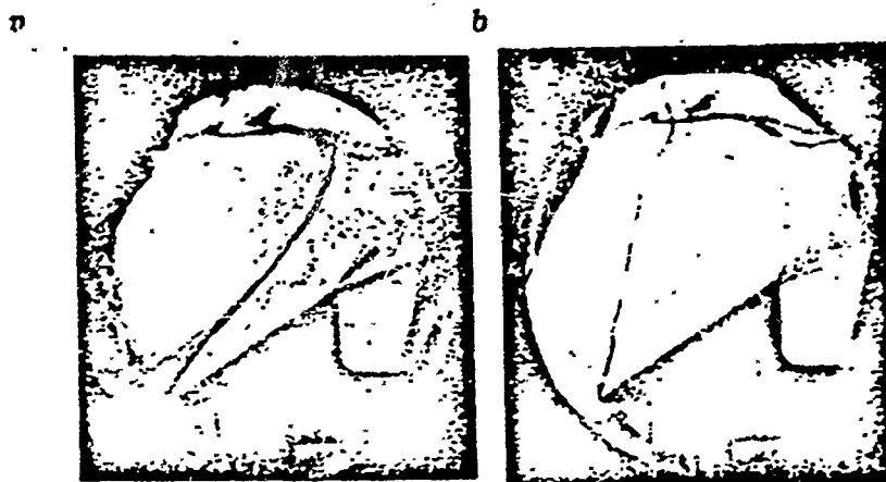
Fig. 17. Arrangement of slanting waves for Ma = 3.0 : a) \bar{Q} = 0 ; b) \bar{Q} = 1.3
