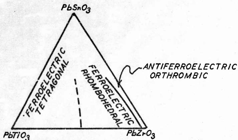
FIG.3 MAJOR PHASES PRESENT IN SYSTEM PbTiO_3 - PbSnO_3 - PbZrO_3
