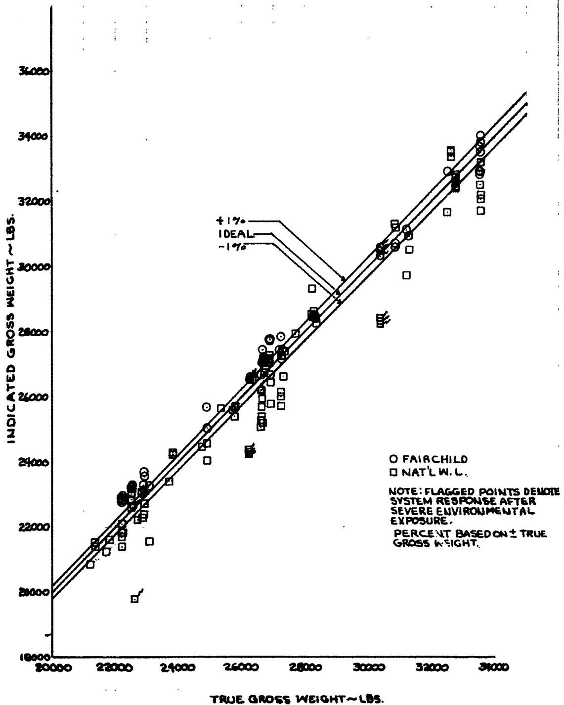
FIGURE No. 2 VARIATION OF INDICATED GROSS WEIGHT CH-47A S/N 468106 STATIC CONDITION
