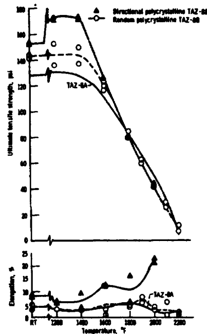
FIGURE 2. TENSILE PROPERTIES OF TAZ-8 ALLOY SERIES(4)
