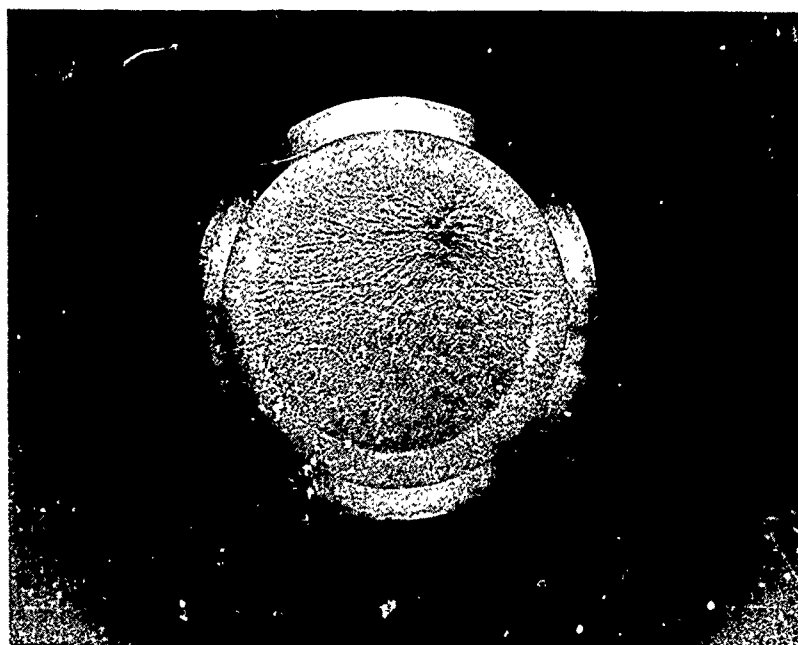
FIGURE 116 FRACTURE SURFACE OF SAMPLE 15, ROUND FRACTURE TOUGHNESS SPECIMEN
