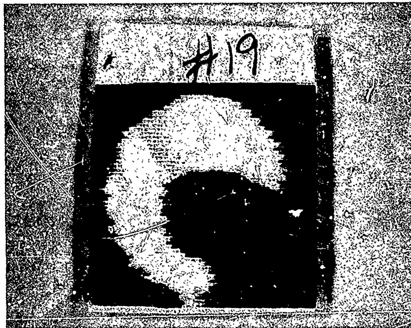
FIGURE 117 "C" SCAN OF INADEQUATELY FATIGUED SPECIMEN, SAMPLE 19
