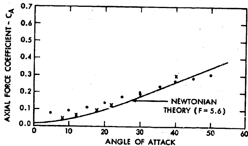
FIG. 48 NORMAL AND AXIAL FORCE COEFFICIENTS - CONFIGURATION 6FX-1
