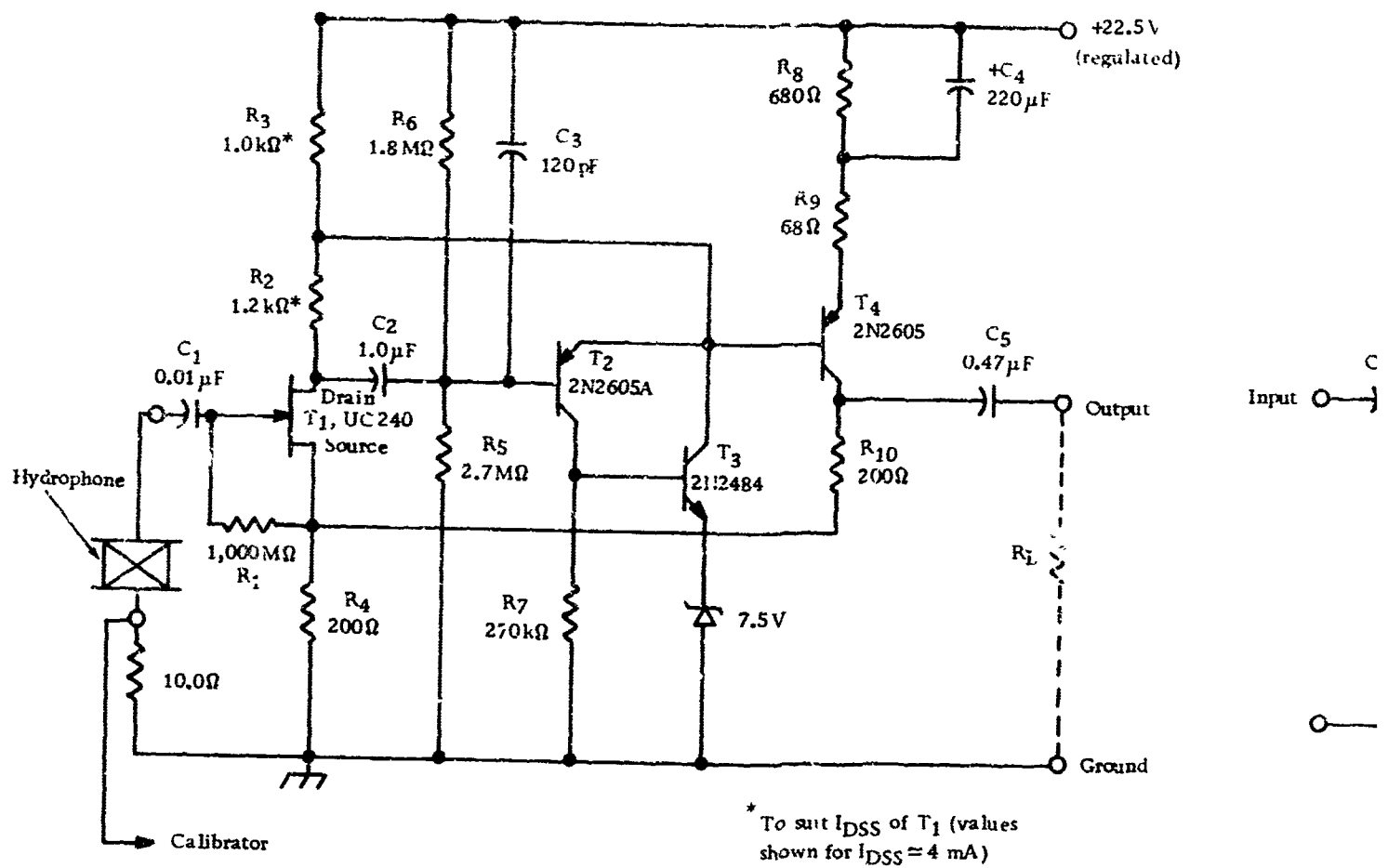
(a) Schematic.
