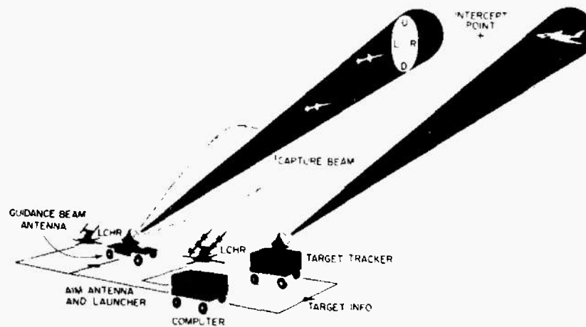
Fig. 5-10 Dual-beam rider.
