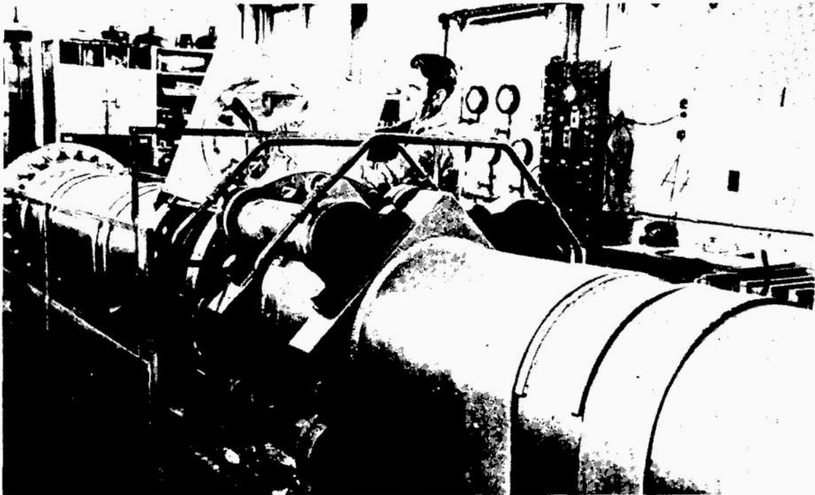
Fig. 6-2 Shock tube.
