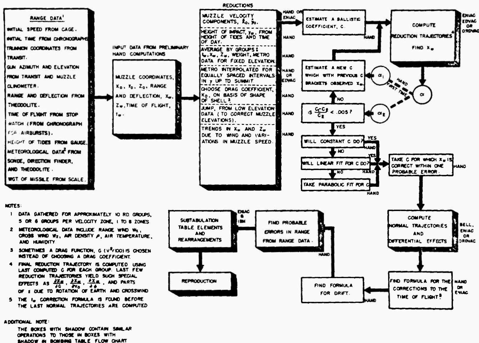
Fig. 3-11 Flow chart for computation of firing tables.
