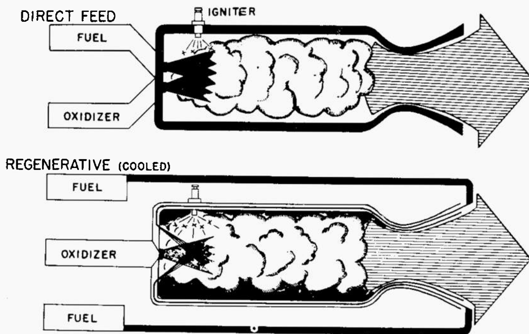
Fig. 2-11 Liquid propellant rocket motor types.
