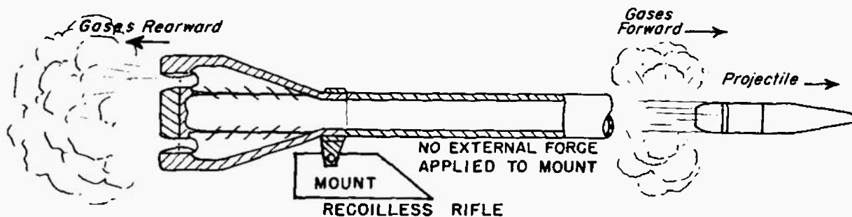
Fig. 1-2 Recoilless system.
