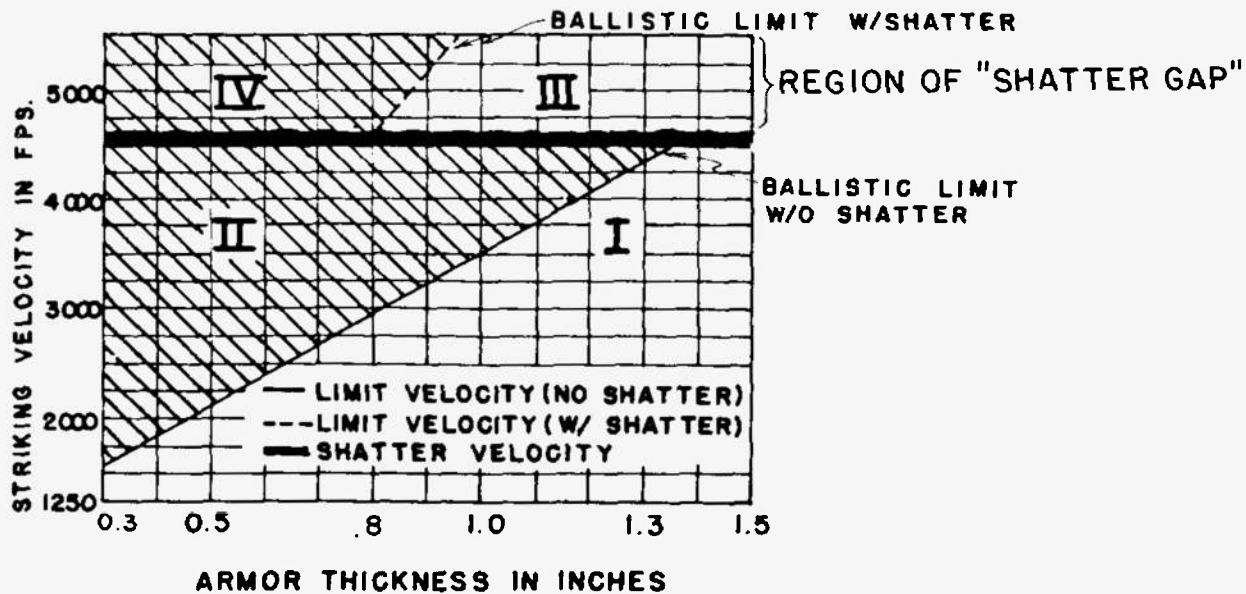
Fig. 10-13 Effect of shatter on perforation.
