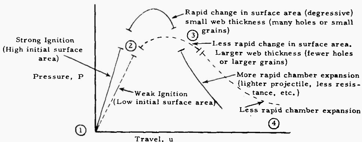
Fig. 1-4 Pressure-travel relationship.
