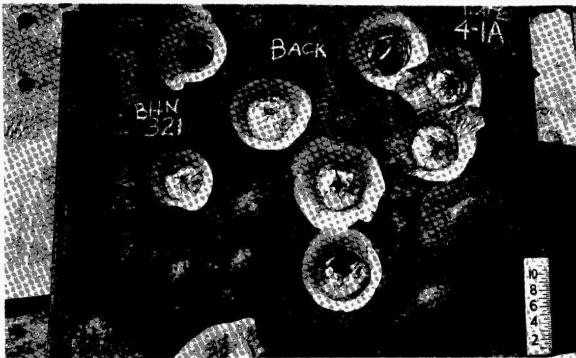
Fig. 10-6 Formation of spall in armor. (Sheet 2 of 2.)
