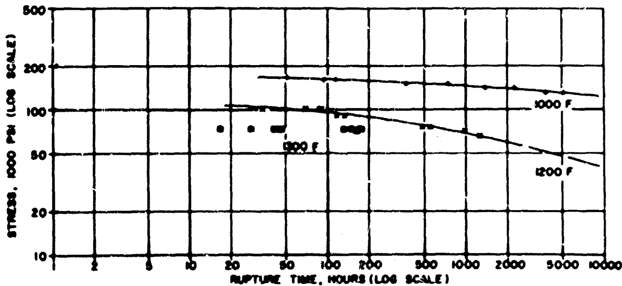
Stress-Rupture Time
