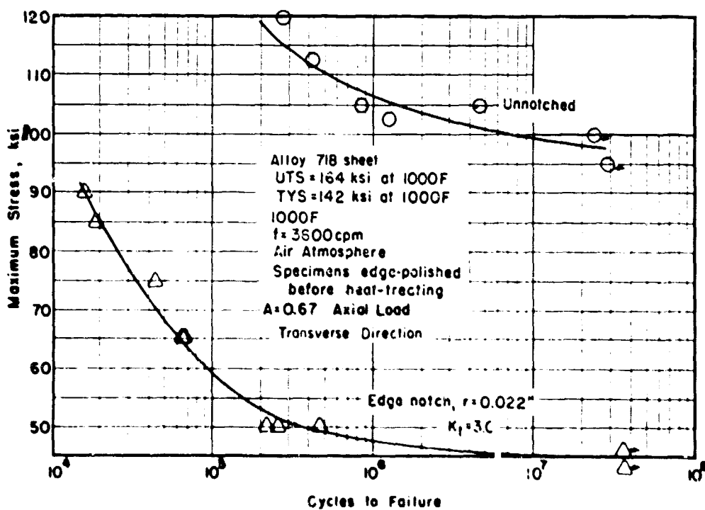
S-N DIAGRAM FOR ALLOY 718 SHEET AT 1000 F WITH STRESS RATIO, A = 0.67 (unnotched and edge-notched)
