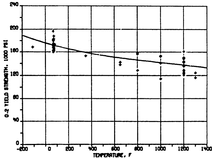
.2% Yield Strength
