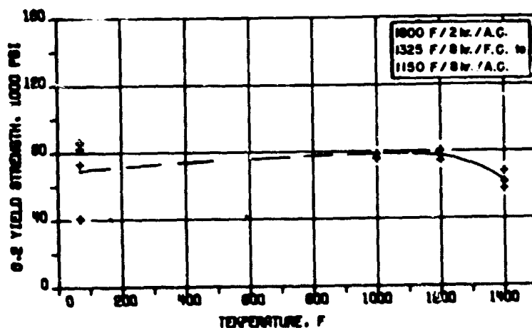
.2% Yield Strength
