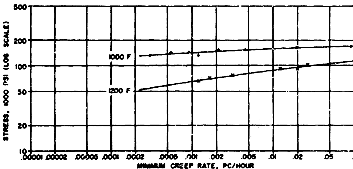
Stress-Creep Rate
