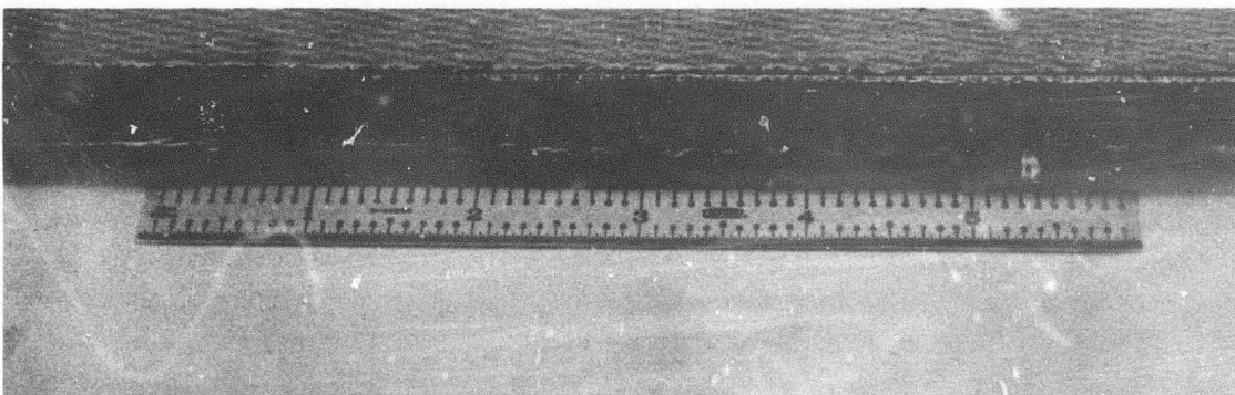
ACCEPTABLE SANDWICH COMPOSITE - AUTOCLAVE PRESSURE - 30 PSI
