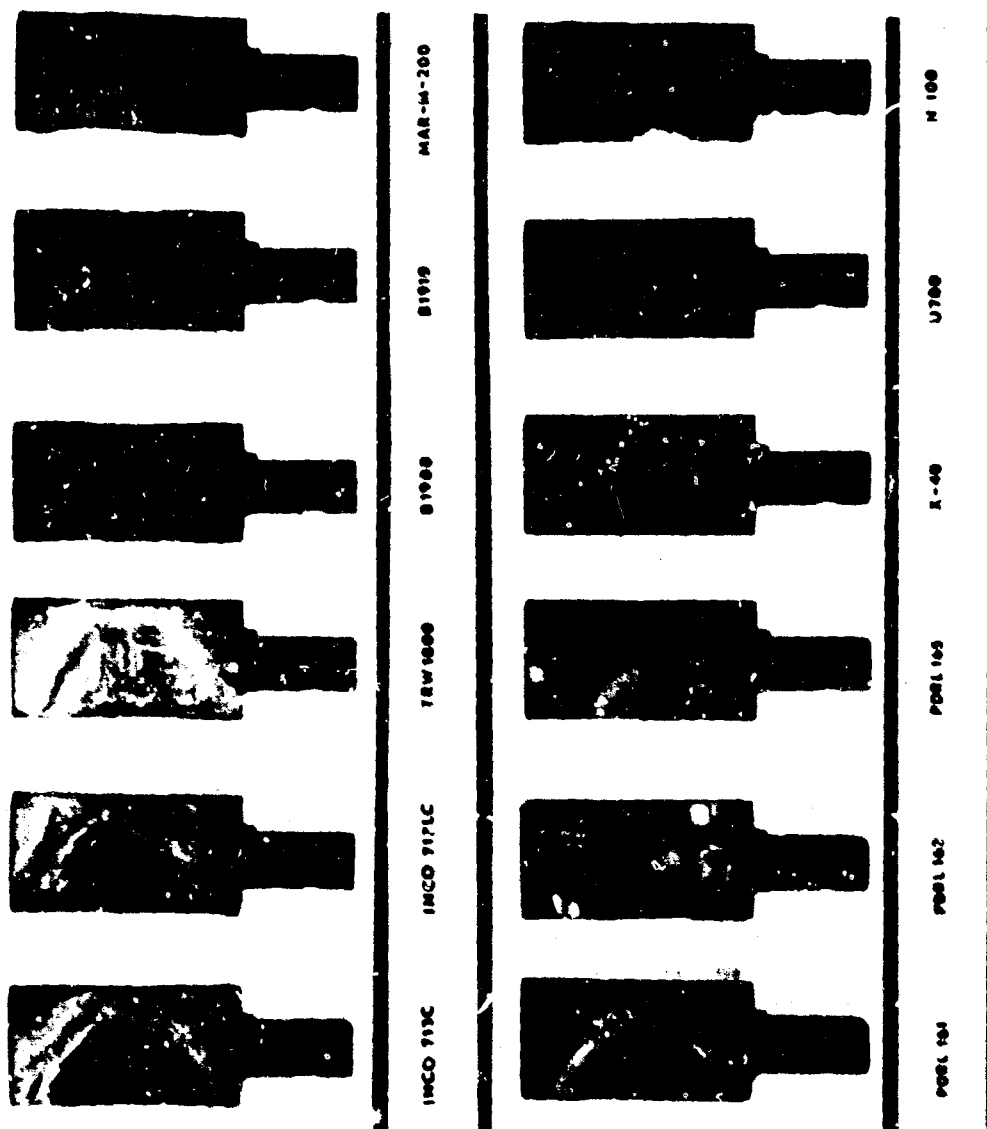
Figure 14. General Appearance of Specimens Tested 120 Hours at 1600°C Using JP-4R Fuel and an 8 ppm Salt/Air Ratio (Test S-530).
